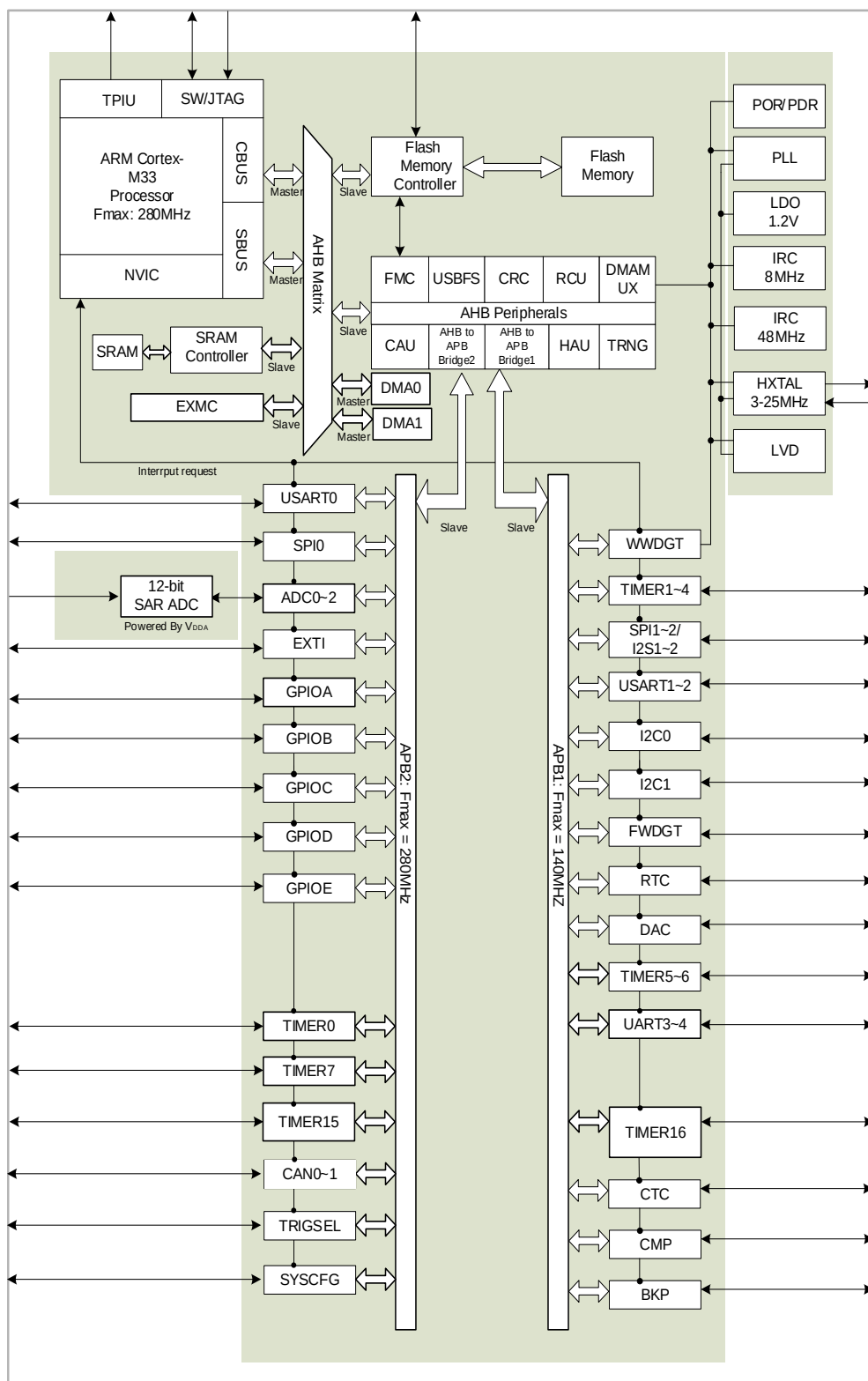
Figure 2-1. GD32F505xx block diagram
