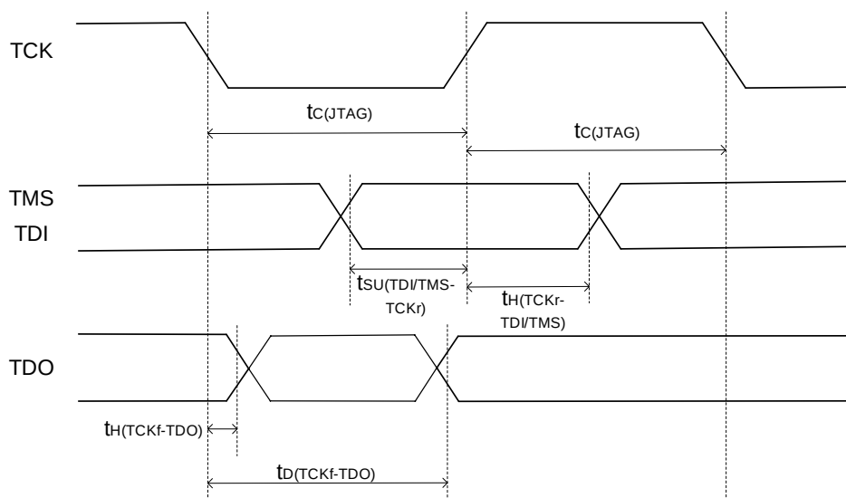
Figure 4-20. JTAG timing diagram
