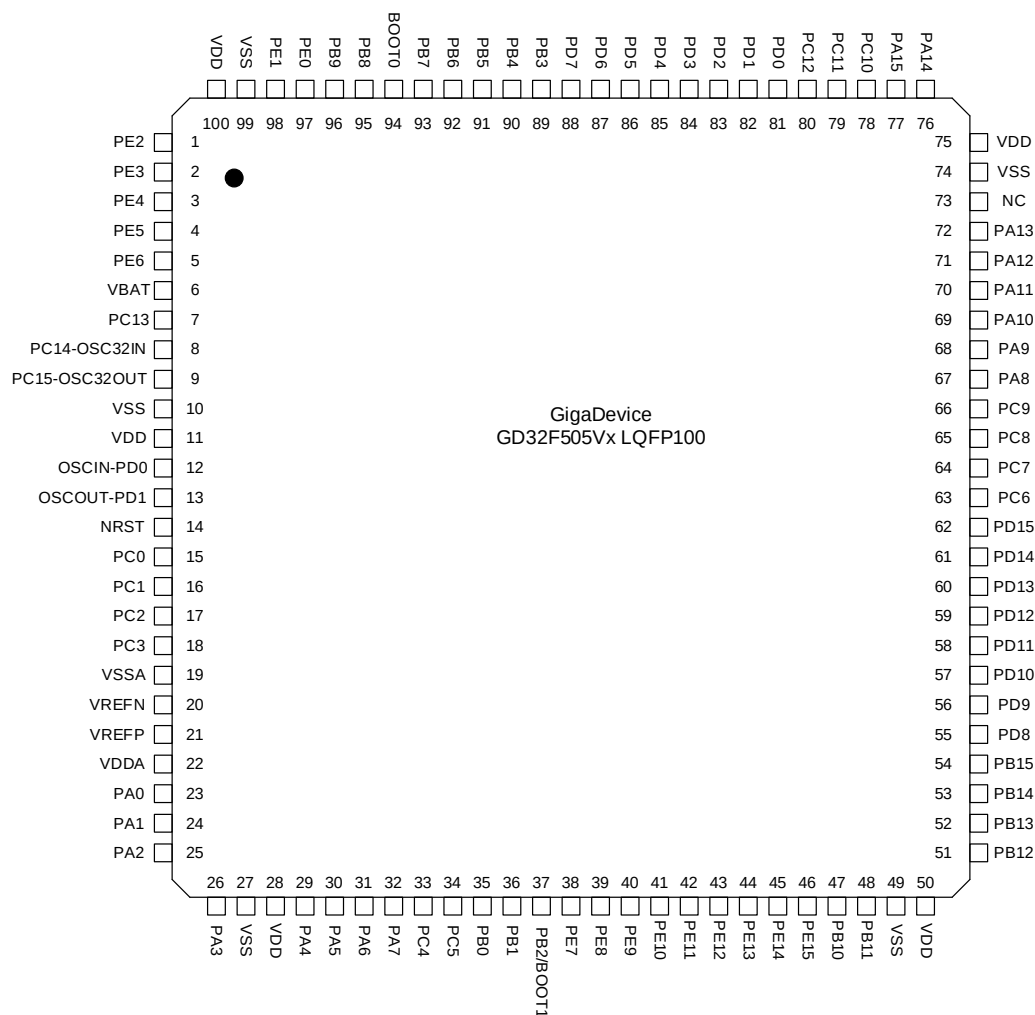
Figure 2-2. GD32F505Vx LQFP100 pinouts
