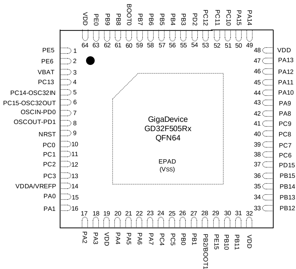
Figure 2-4. GD32F505Rx QFN64 pinouts
