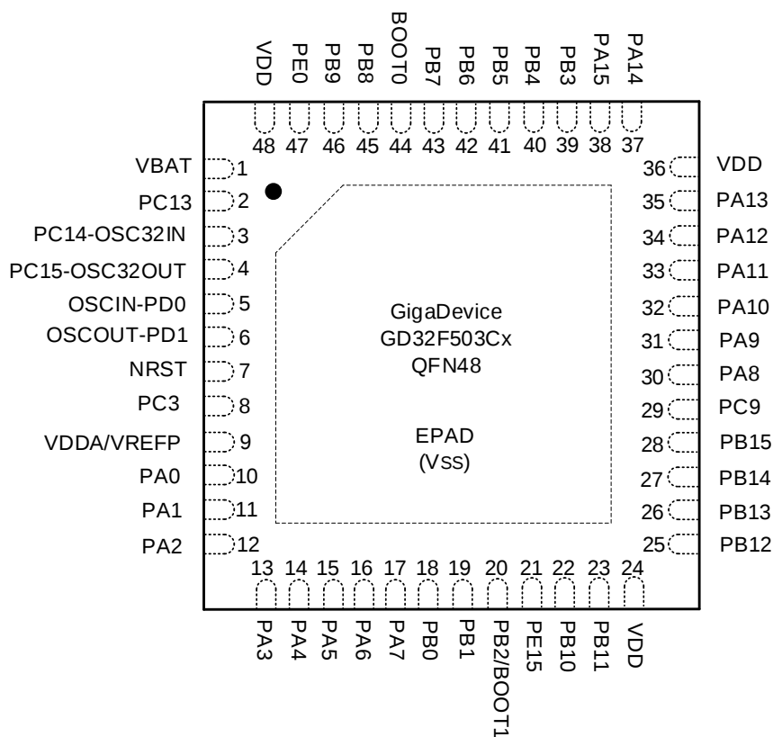
Figure 2-7. GD32F503Cx QFN48 pinouts
