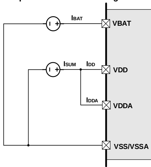
Figure 4-3. Power consumption measurement diagram
