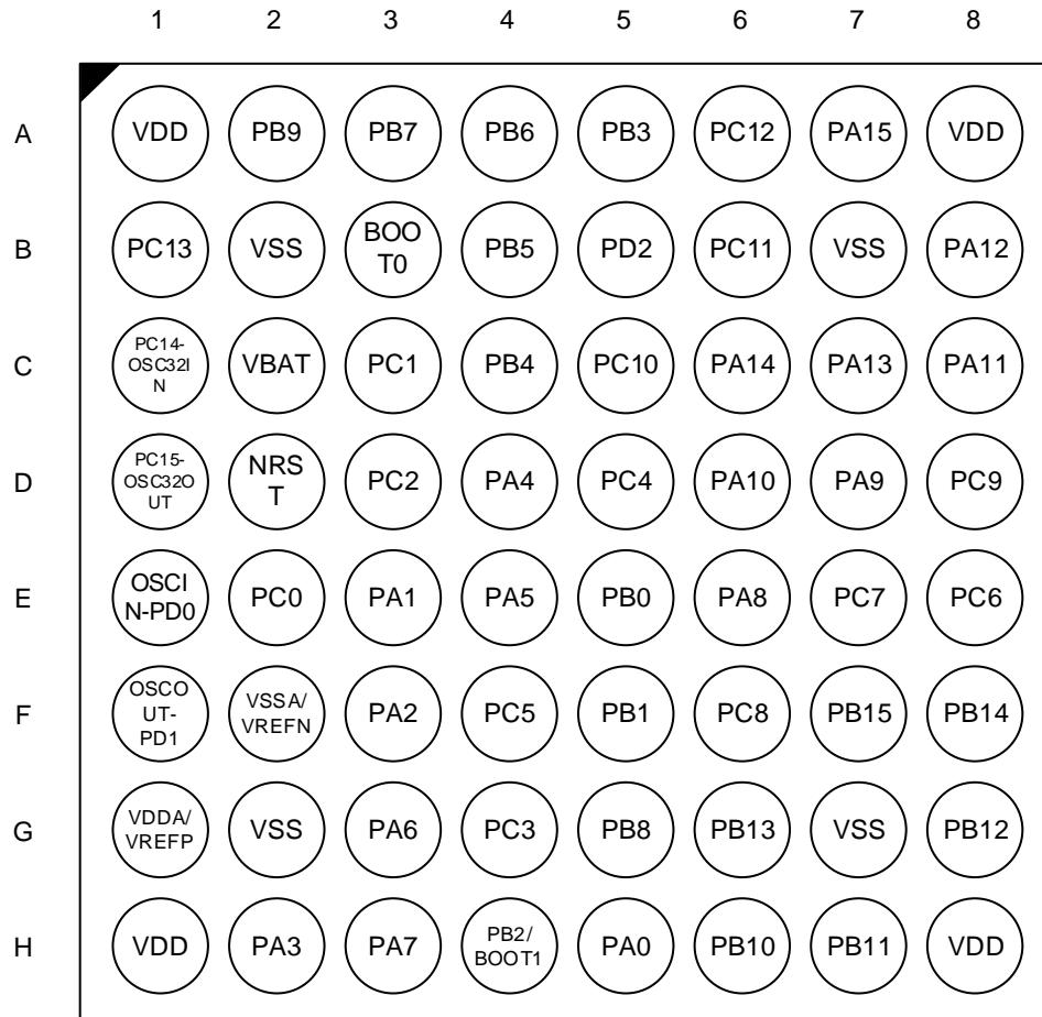
Figure 2-5. GD32F502Rx BGA64 pinouts
