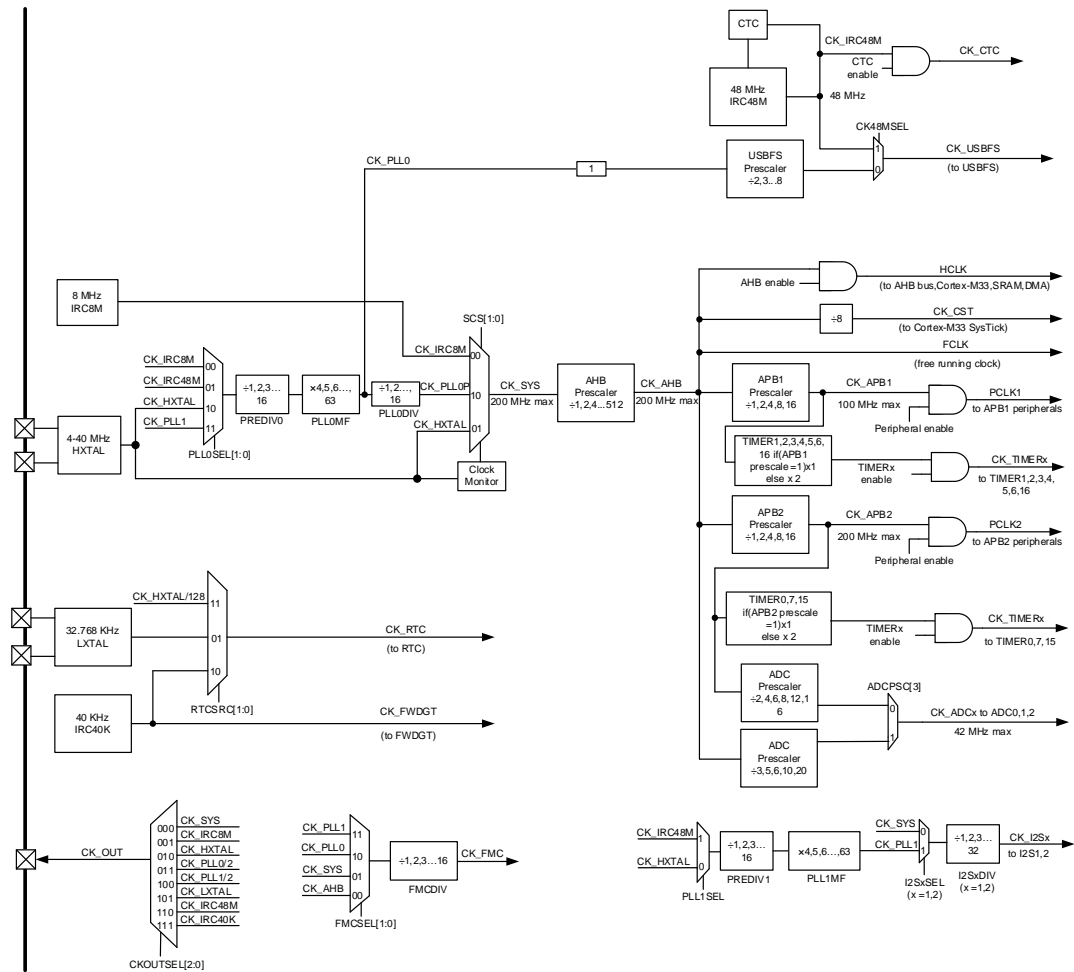
Figure 2-9. GD32F502xx clock tree
