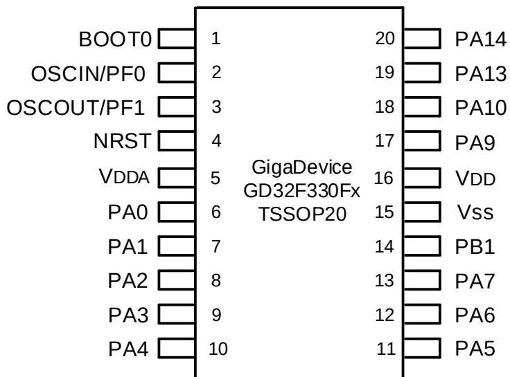
Figure 2-7. GD32F330Fx TSSOP20 pinouts
