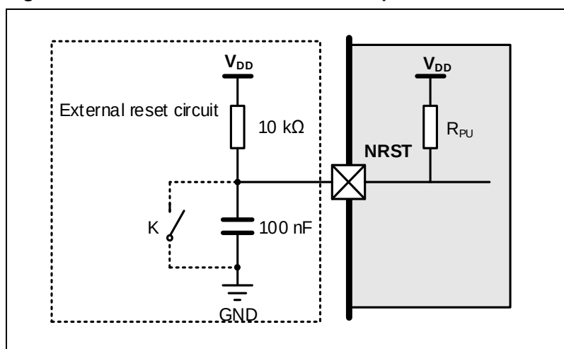
Figure 4-4. Recommended external NRST pin circuit (1)
