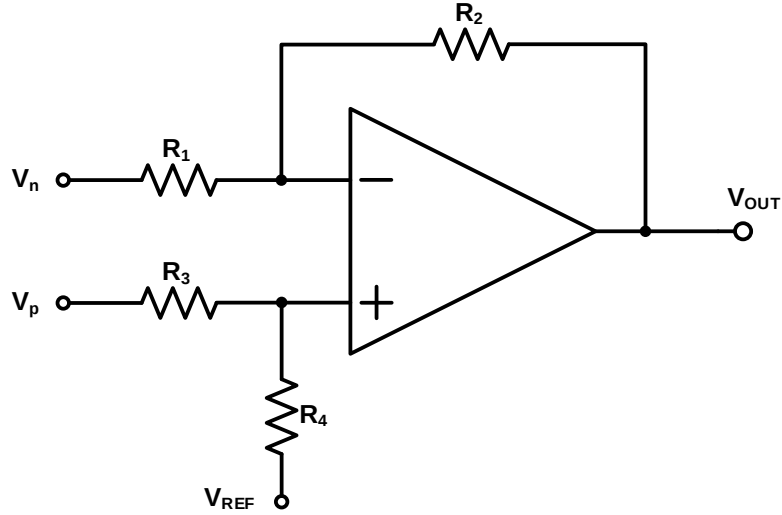
Figure 22. Differential Amplifier
