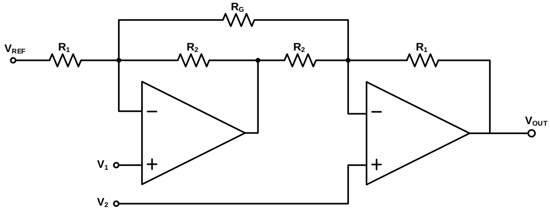
Figure 23. Instrumentation Amplifier
