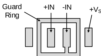
Figure 18. Use a Guard Ring around Sensitive Pins
