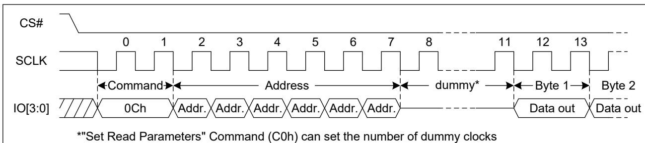
Figure 36. Burst Read with Wrap Sequence Diagram
