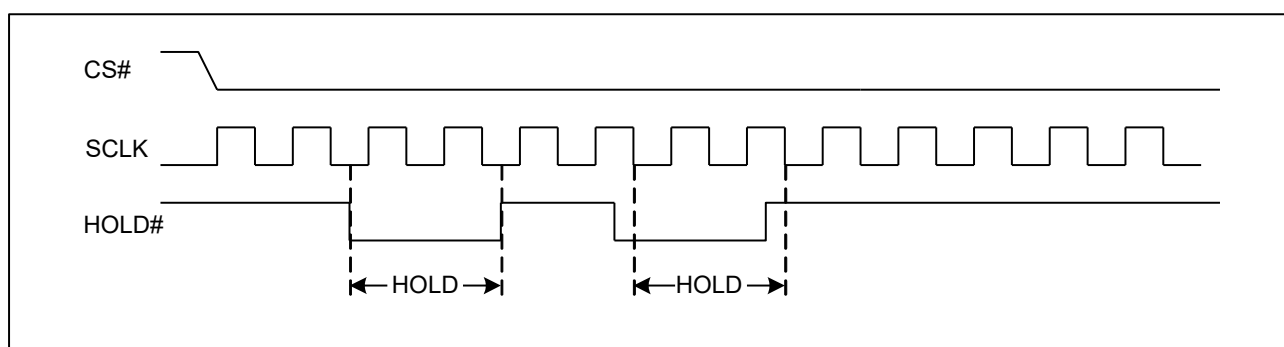
Figure 3 HOLD Condition
