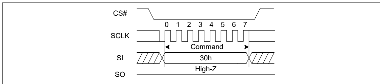
Figure 19. Clear Status Register Flags Sequence Diagram
