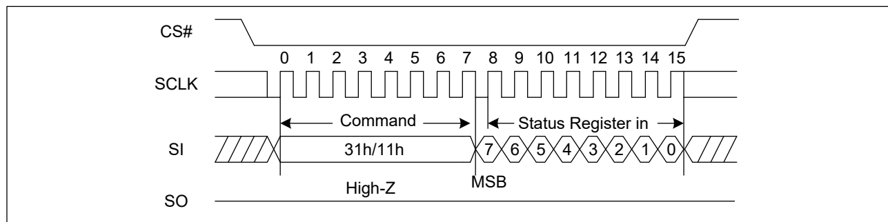
Figure 15. Write Status Register Sequence Diagram (SPI)
