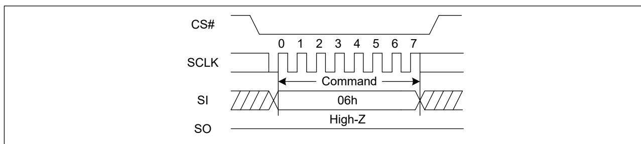
Figure 7. Write Enable Sequence Diagram (SPI)
