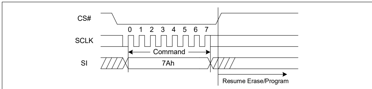
Figure 63. Program/Erase Resume Sequence Diagram (SPI)
