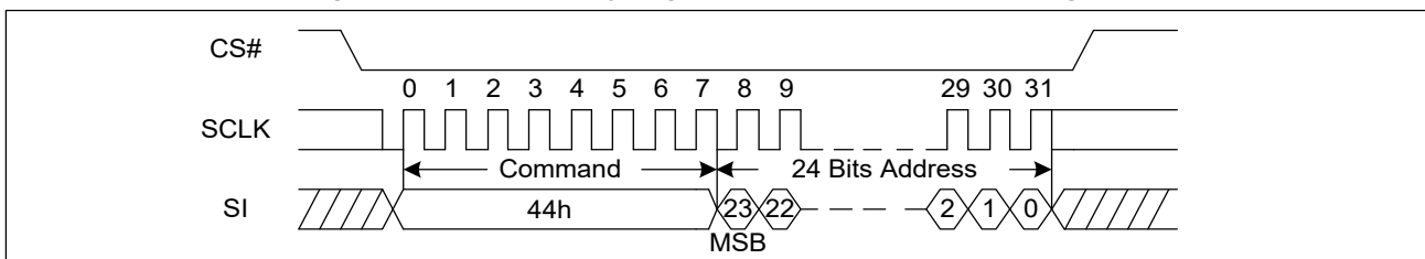
Figure 56. Erase Security Registers command Sequence Diagram
