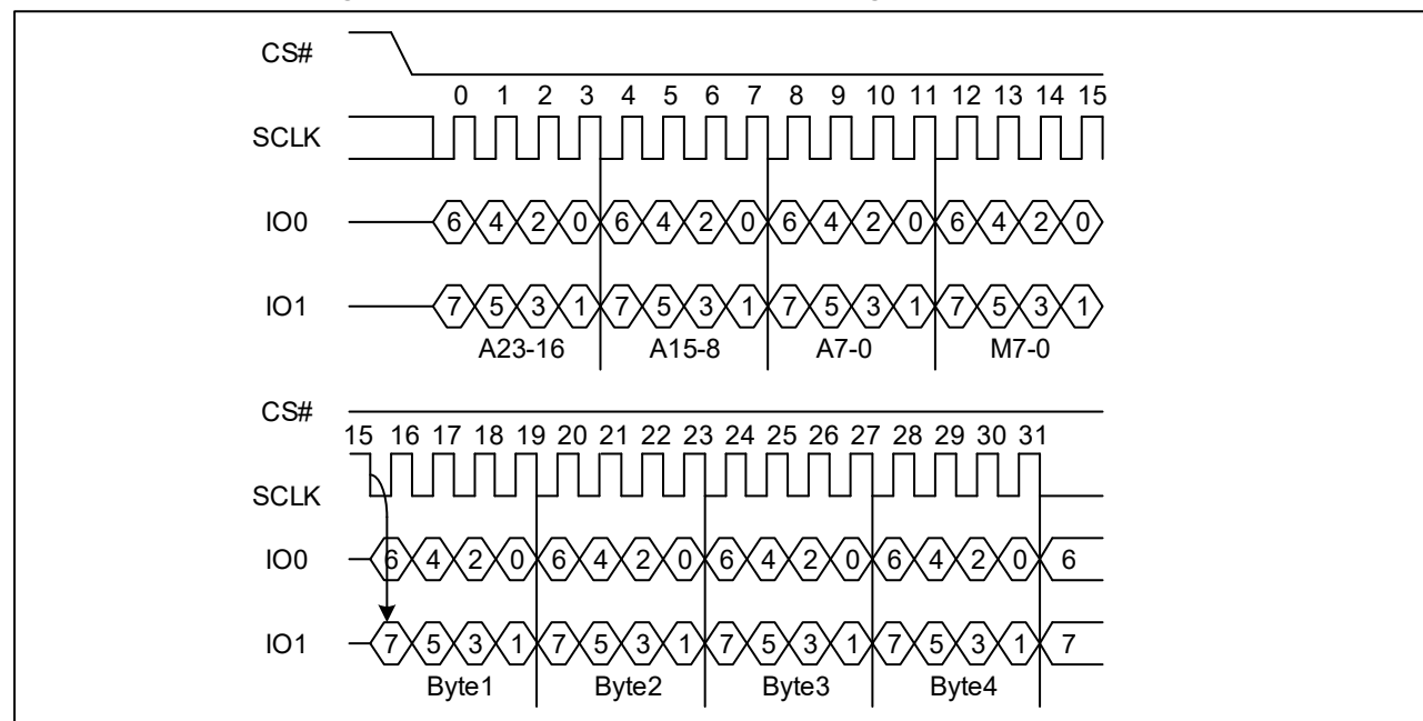
Figure 26. Dual I/O Fast Read Sequence Diagram ((M5-4) = (1, 0))
