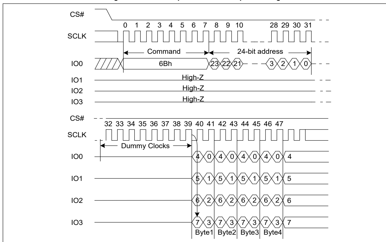
Figure 29. Quad Output Fast Read Sequence Diagram
