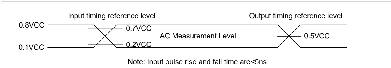
Figure 76. Absolute Maximum Ratings Diagram
