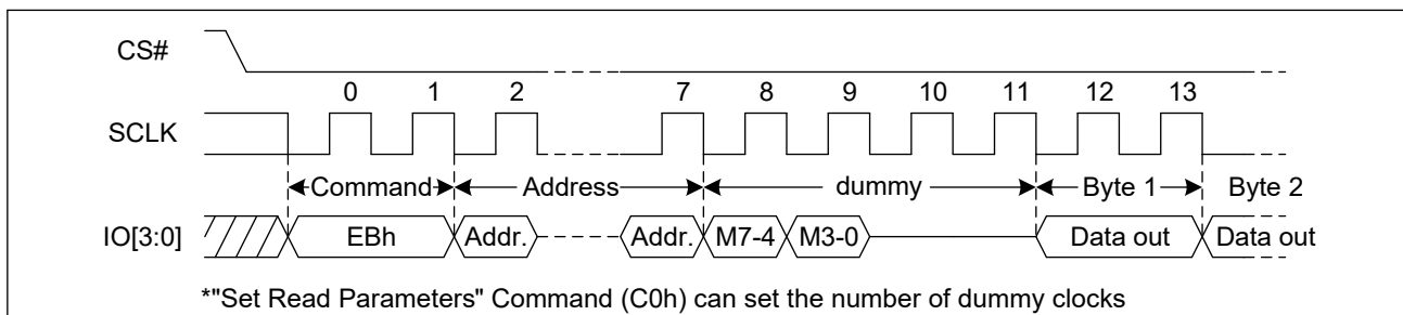
Figure 31. Quad I/O Fast Read Sequence Diagram ((M5-4) ≠ (1, 0), QPI)
