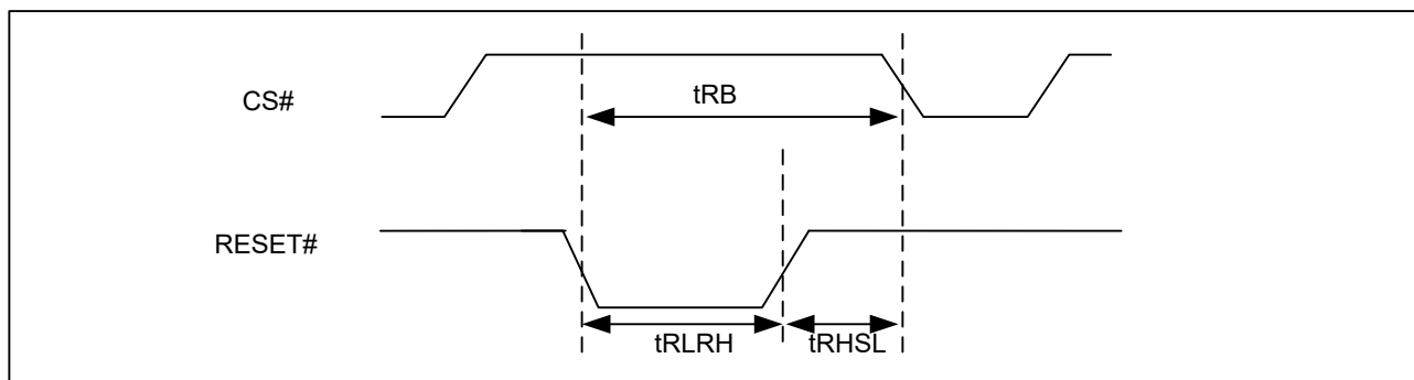
Figure 84. RESET# Timing
