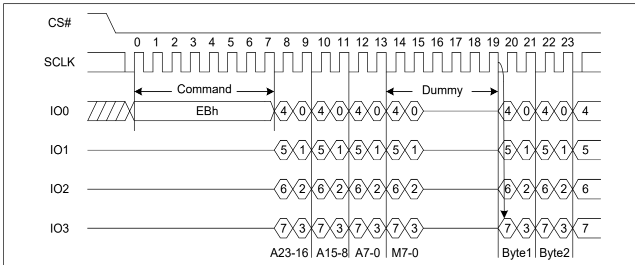
Figure 30. Quad I/O Fast Read Sequence Diagram ((M5-4) ≠ (1, 0), SPI)
