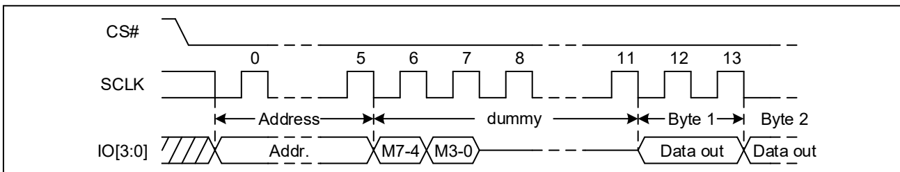
Figure 32. Quad I/O Fast Read Sequence Diagram ((M5-4) = (1, 0))
