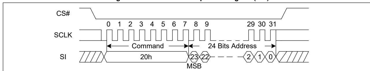
Figure 43. Sector Erase Sequence Diagram (SPI)
