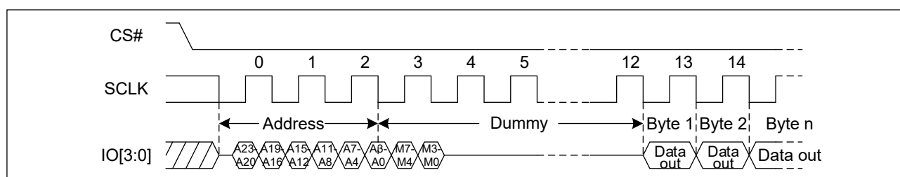
Figure 35. DTR Quad I/O Fast Read Sequence Diagram (M5-4 = (1, 0))
