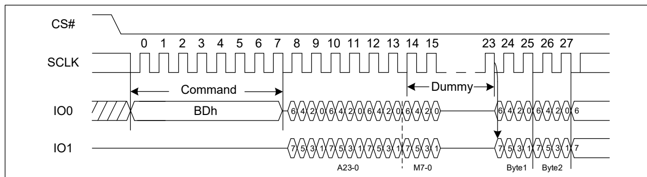
Figure 27. DTR Dual I/O Fast Read Sequence Diagram (M5-4 ≠ (1, 0))
