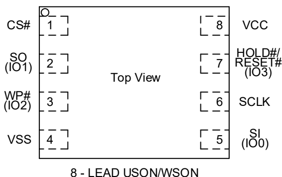
Figure 1 Connection Diagram for USON8/WSO8 package
