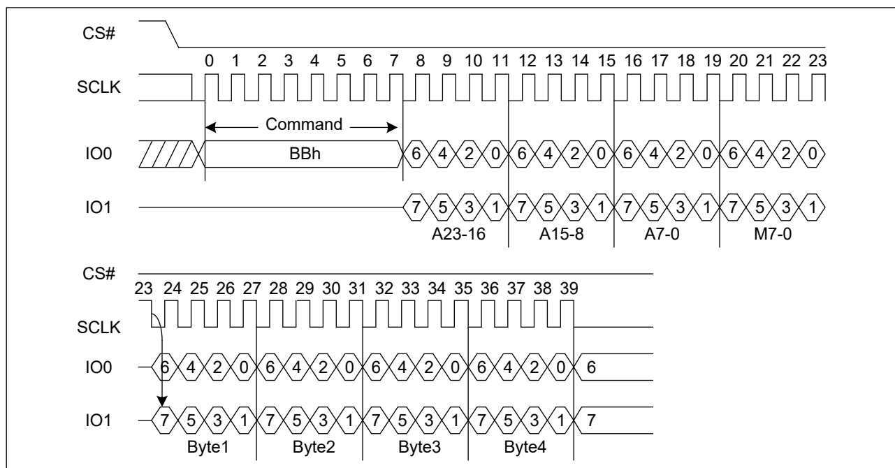
Figure 25. Dual I/O Fast Read Sequence Diagram ((M5-4) ≠ (1, 0))
