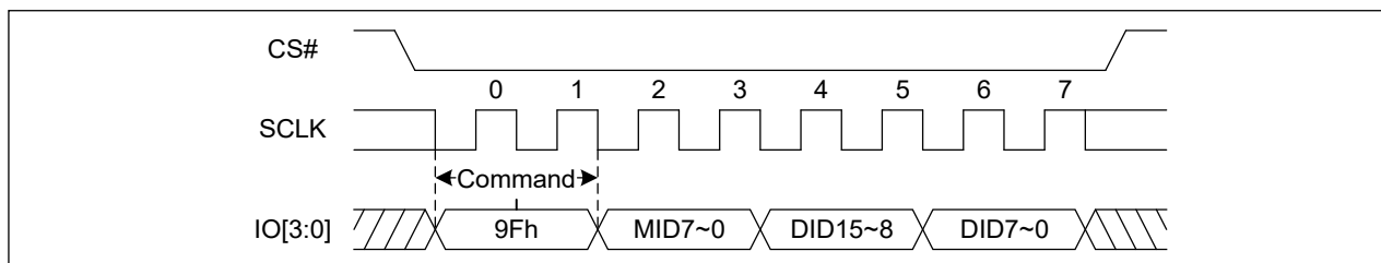
Figure 54. Read Identification ID Sequence Diagram (QPI)
