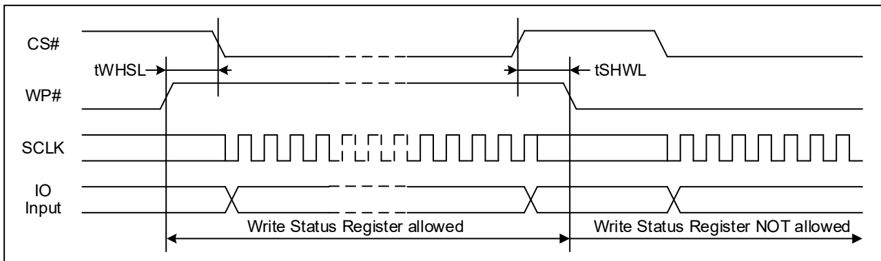
Figure 82. WP# Timing
