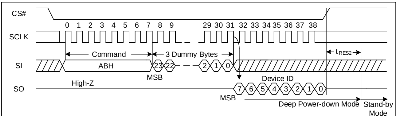
Figure 63. Release Power-Down/Read Device ID Sequence Diagram (SPI)
