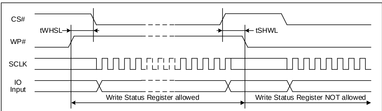
Figure 104. WP# Timing
