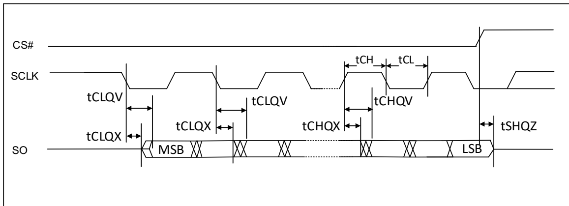
Figure 24-4. Serial Output Timing (DTR)
