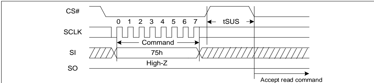
Figure 53. Program/Erase Suspend Sequence Diagram (SPI)
