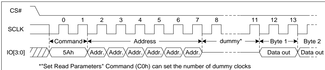
Figure 66. Read Serial Flash Discoverable Parameter command Sequence Diagram (QPI)
