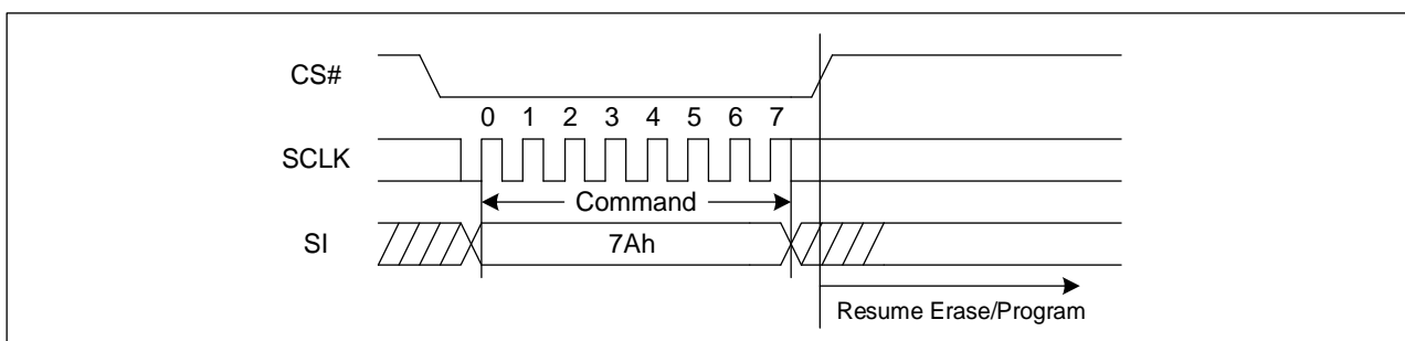
Figure 55. Program/Erase Resume Sequence Diagram (SPI)
