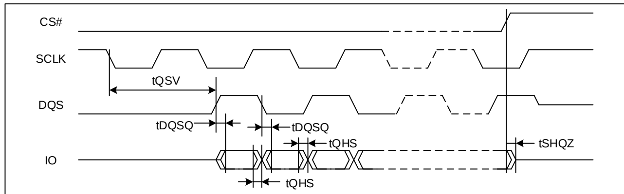
Figure 125. DQS Output Timing (DTR)
