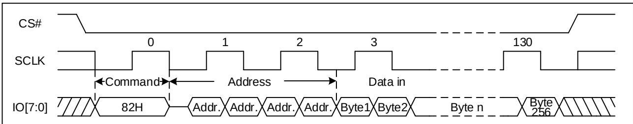
Figure 61. Page Program Sequence Diagram (DTR OPI)
