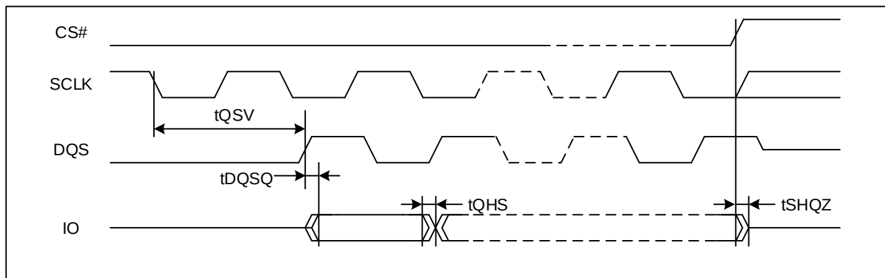
Figure 124. DQS Output Timing (STR)
