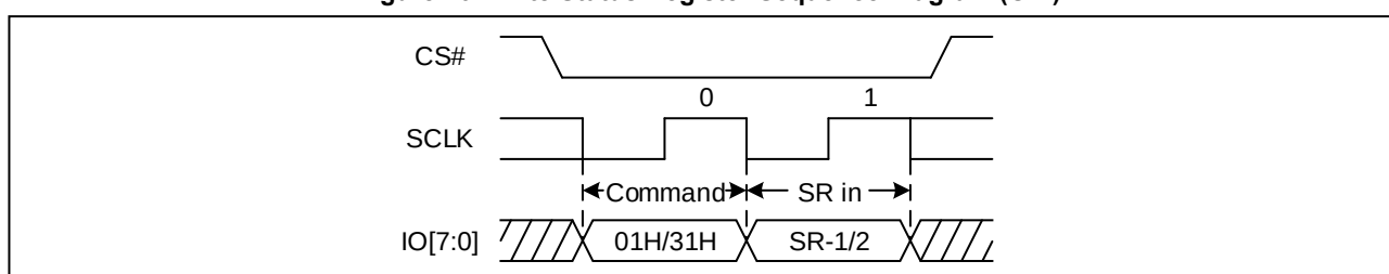
Figure 26. Write Status Register Sequence Diagram (OPI)
