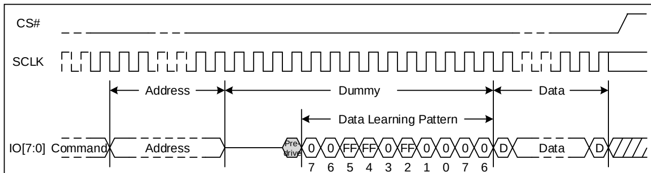
Figure 11. Data Learning Pattern Sequence Diagram (STR, Dummy Clock \geq 12 )
