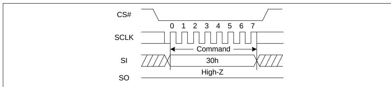
Figure 39. Clear Status Register Flags Sequence Diagram
