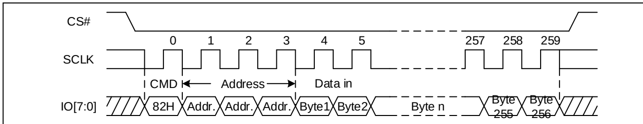
Figure 60. Page Program Sequence Diagram (STR OPI)
