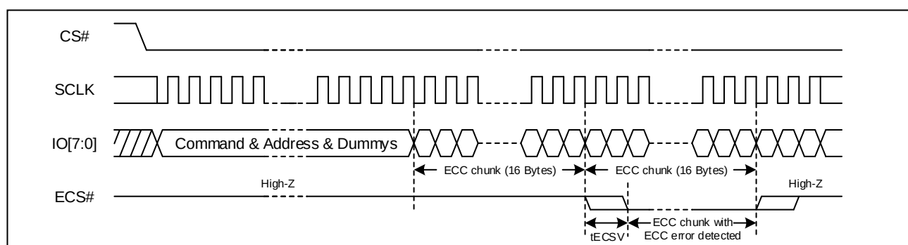
Figure 3. ECS# Timing
