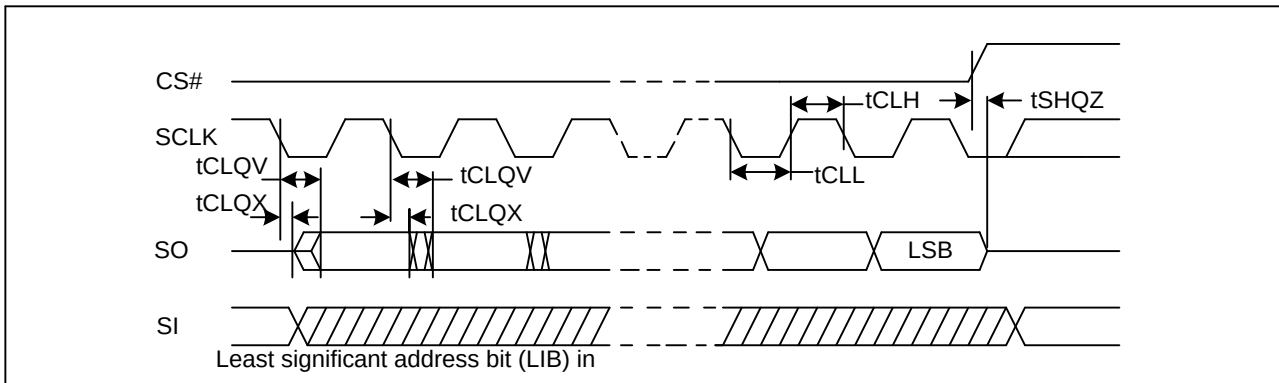
Figure 121. Output Timing
