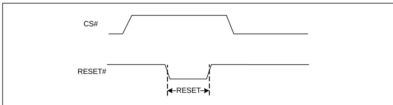
Figure 2 RESET Condition
