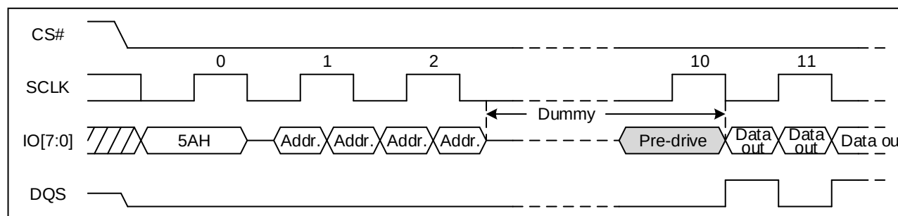
Figure 116. Read Serial Flash Discoverable Parameter command Sequence Diagram (DTR OPI)
