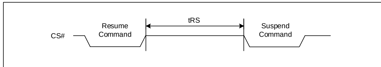
Figure 126. Resume to Suspend Timing Diagram
