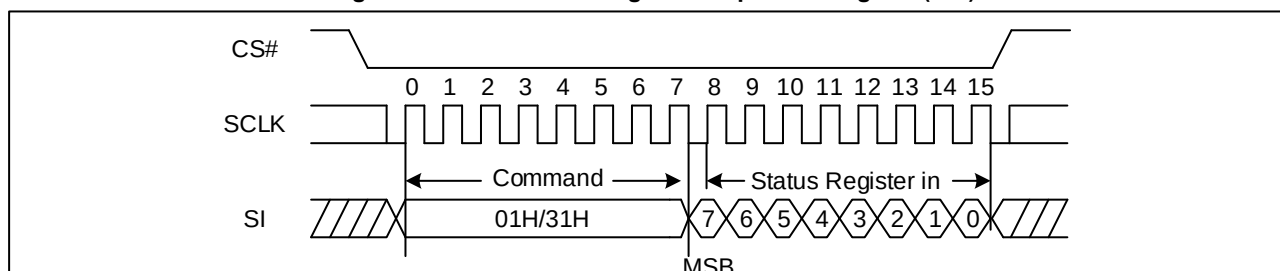
Figure 25. Write Status Register Sequence Diagram (SPI)
