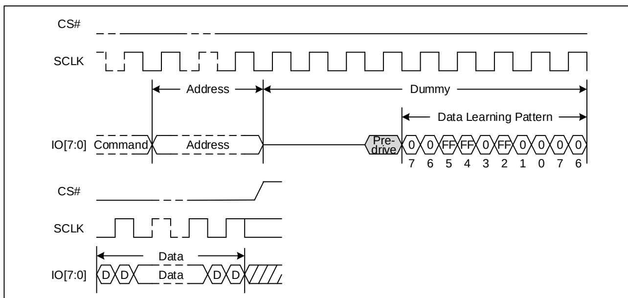
Figure 13. Data Learning Pattern Sequence Diagram (DTR, Dummy Clock \geq 8 )
