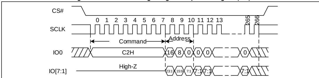
Figure 62. Extend Octal Page Program Sequence Diagram (SPI)
