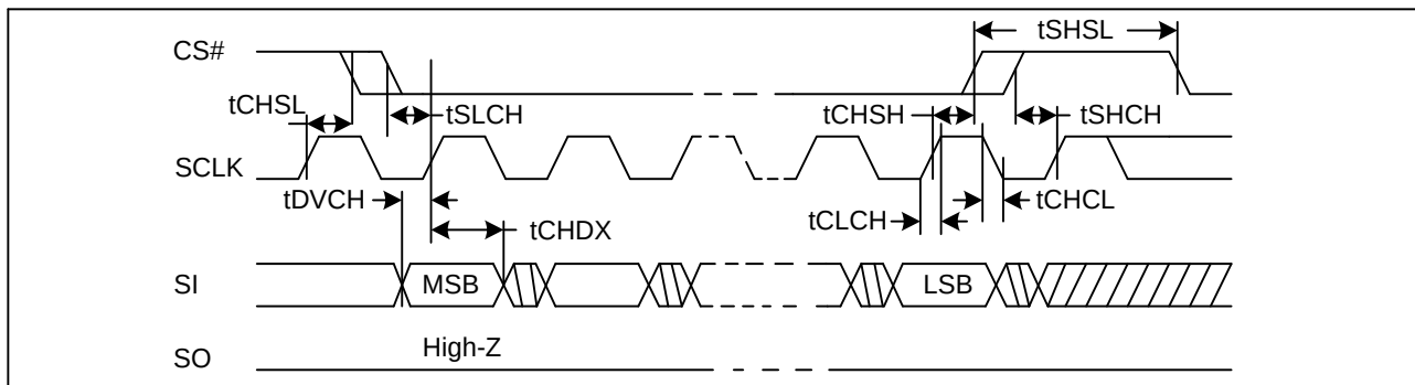
Figure 43. Input Timing
