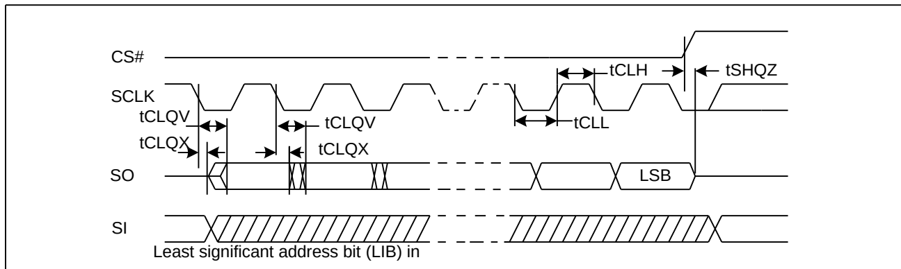
Figure 44. Output Timing
