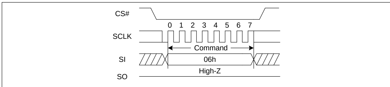
Figure 5. Write Enable Sequence Diagram
