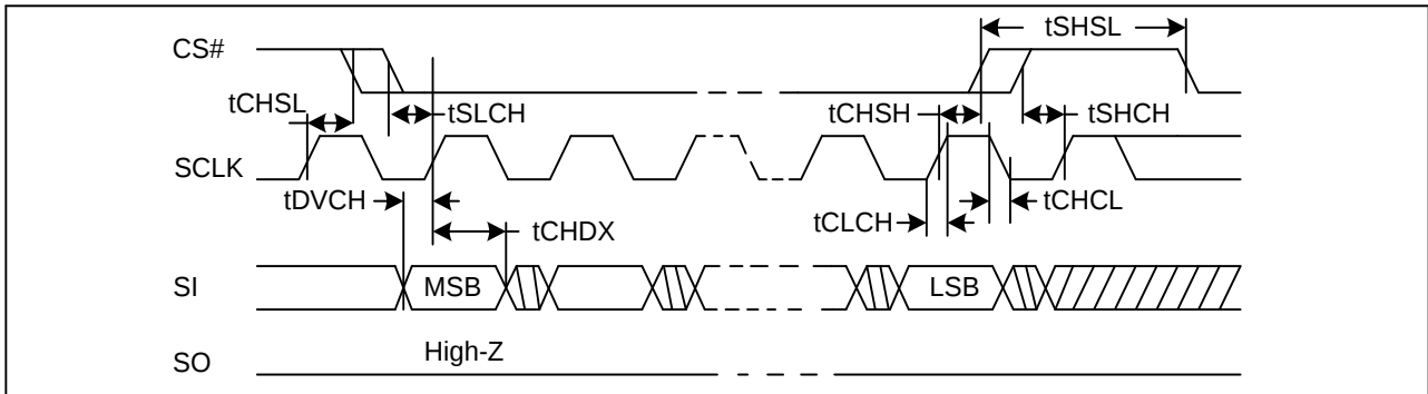
Figure 44. Input Timing
