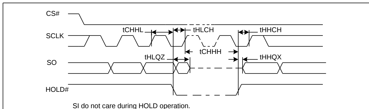
Figure 49. Hold Timing
