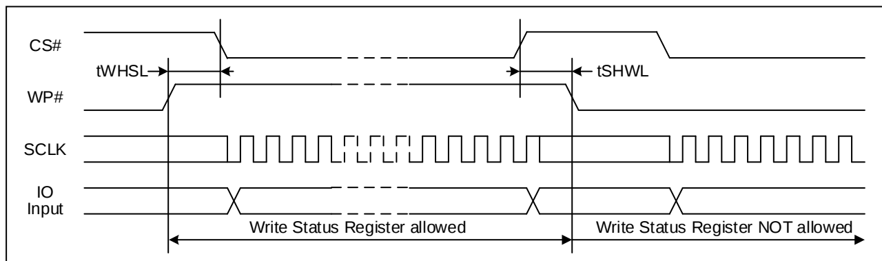
Figure 50. WP# Timing
