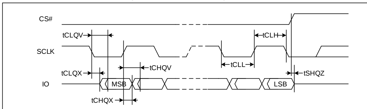
Figure 47. Serial Output Timing (DTR)
