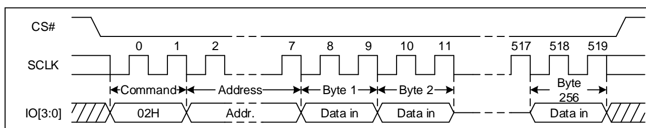
Figure 47 Page Program Sequence Diagram (QPI)
