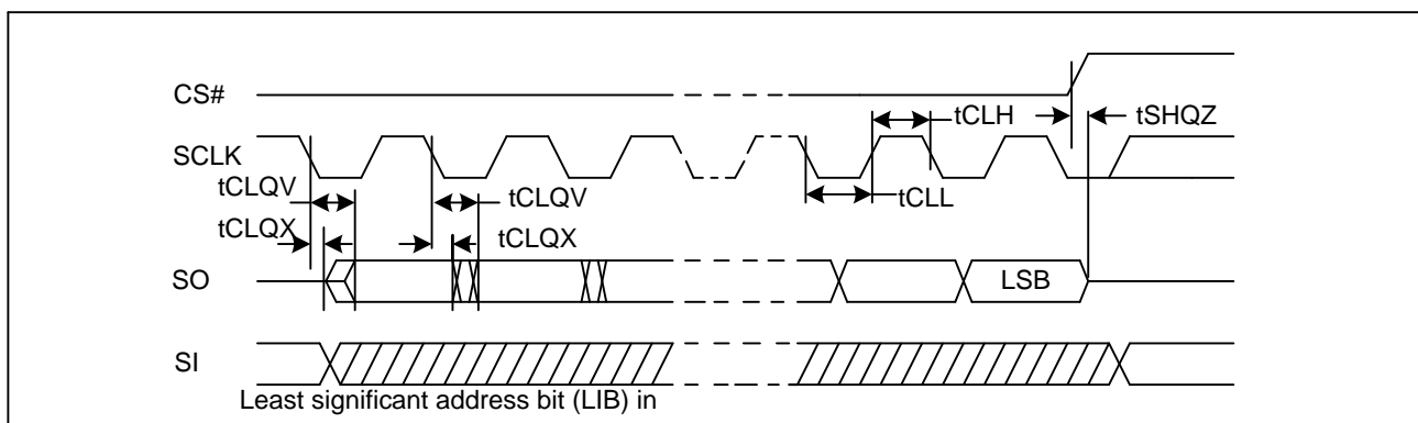
Figure 98. Output Timing
