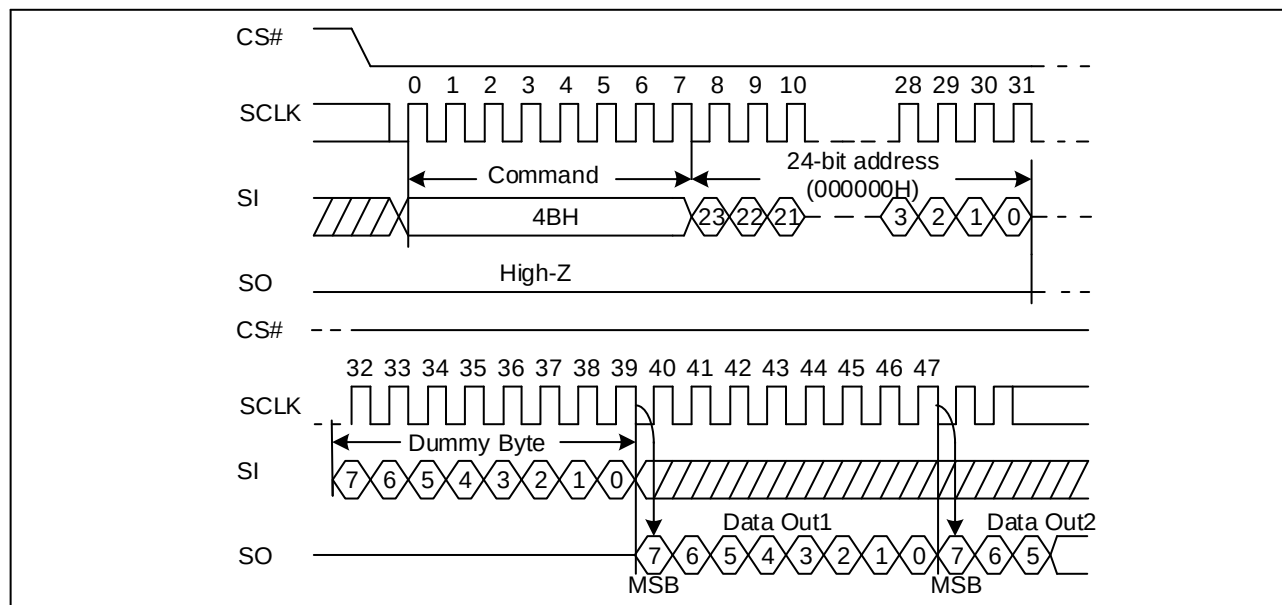
Figure 4 Read Unique ID Sequence Diagram (SPI)
