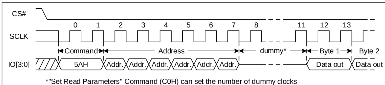
Figure 93 Read Serial Flash Discoverable Parameter command Sequence Diagram (QPI)
