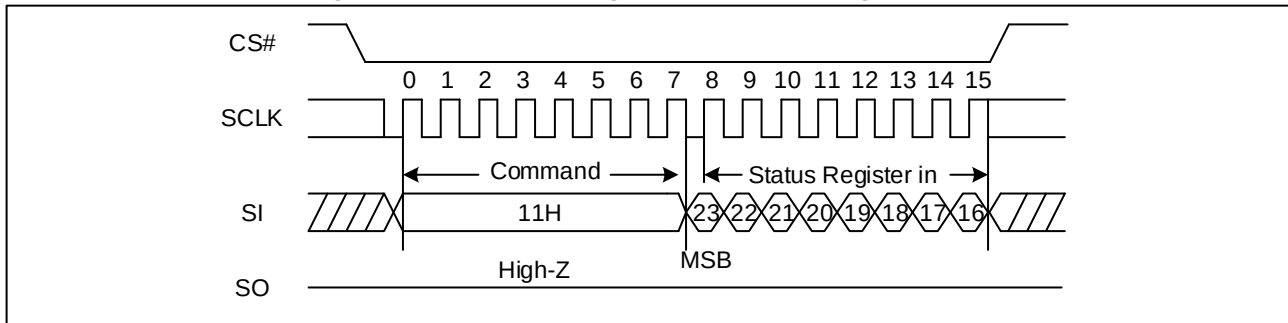
Figure 19. Write Status Register-3 Sequence Diagram (SPI)
