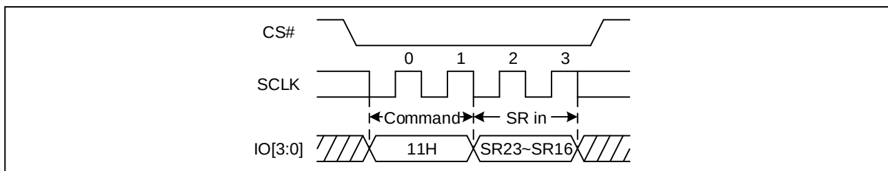
Figure 20. Write Status Register-3 Sequence Diagram (QPI)
