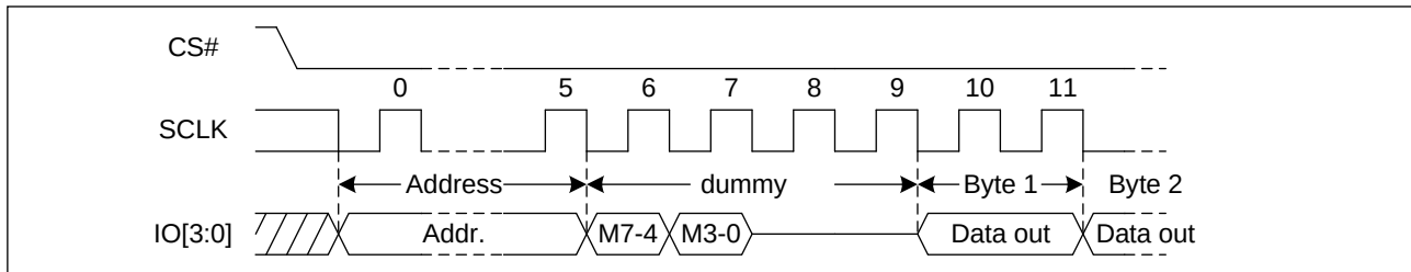
Figure 42 Quad I/O Fast Read Sequence Diagram (M5-4= (1, 0))
