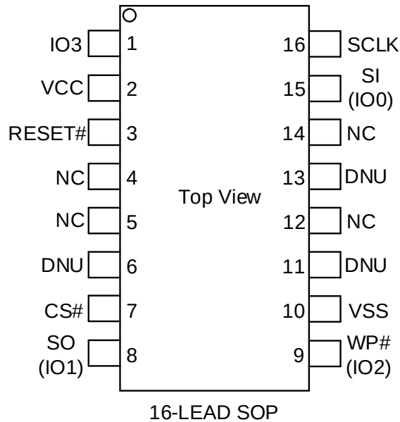
Figure 2 Connection Diagram for SOP16 package
