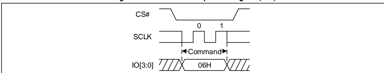
Figure 13 Write Enable Sequence Diagram (QPI)
