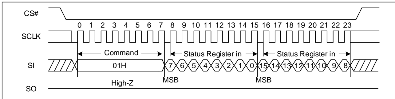
Figure 20. Write Status Register-1&2 Sequence Diagram (SPI)
