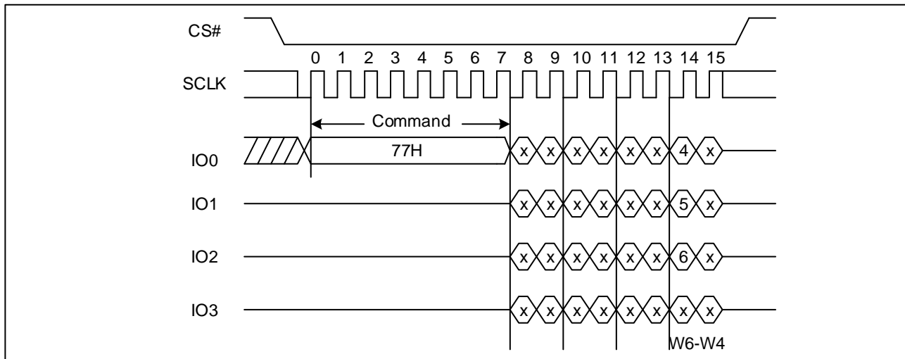
Figure 45. Set Burst with Wrap Sequence Diagram
