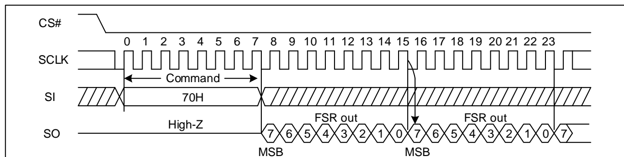
Figure 28 Read Flag Status Register Sequence Diagram (SPI)
