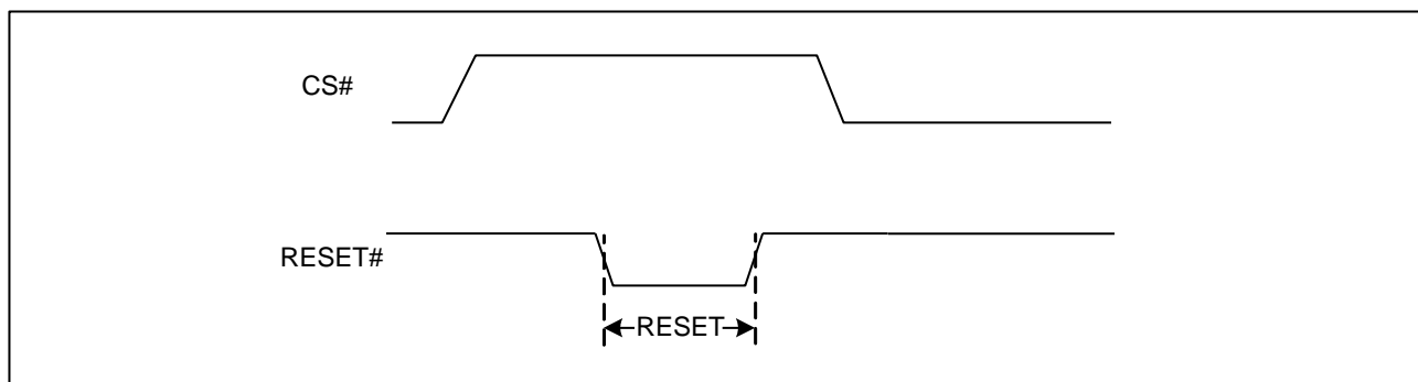
Figure 3 RESET Condition
