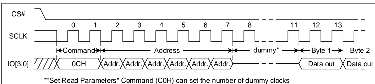
Figure 44. Burst Read with Wrap Sequence Diagram
