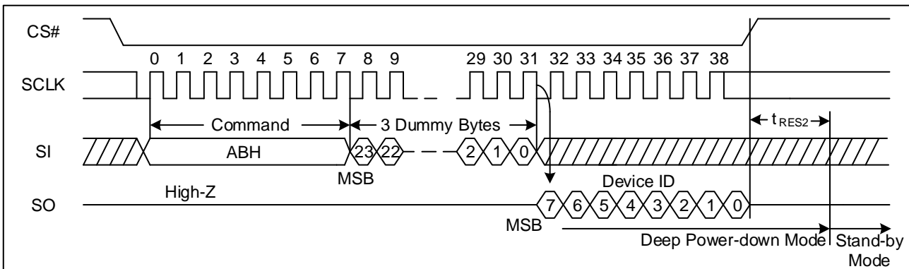
Figure 64. Release Power-Down/Read Device ID Sequence Diagram (SPI)
