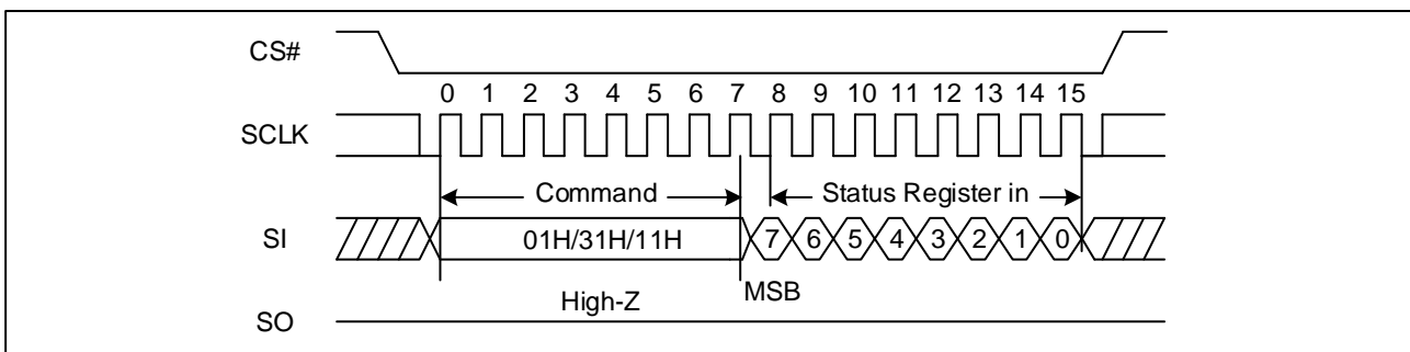
Figure 18 Write Status Register Sequence Diagram (SPI)
