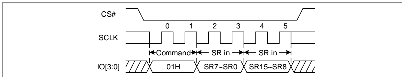
Figure 22. Write Status Register-1&2 Sequence Diagram (QPI)
