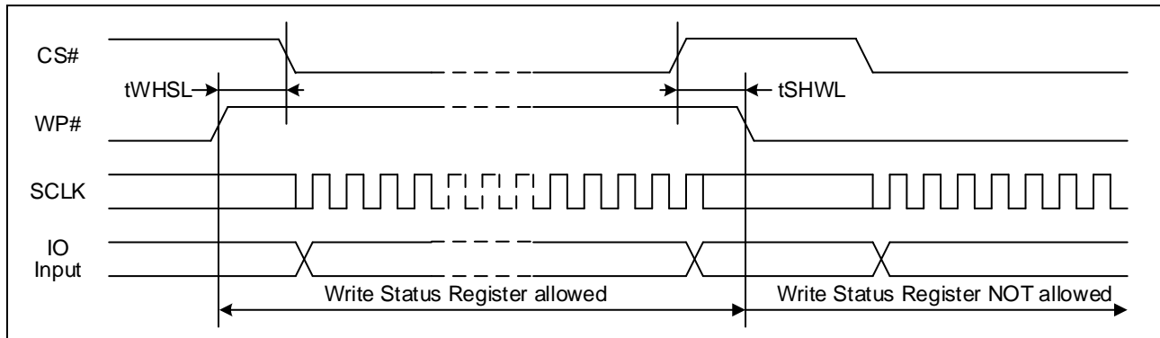
Figure 101. WP# Timing
