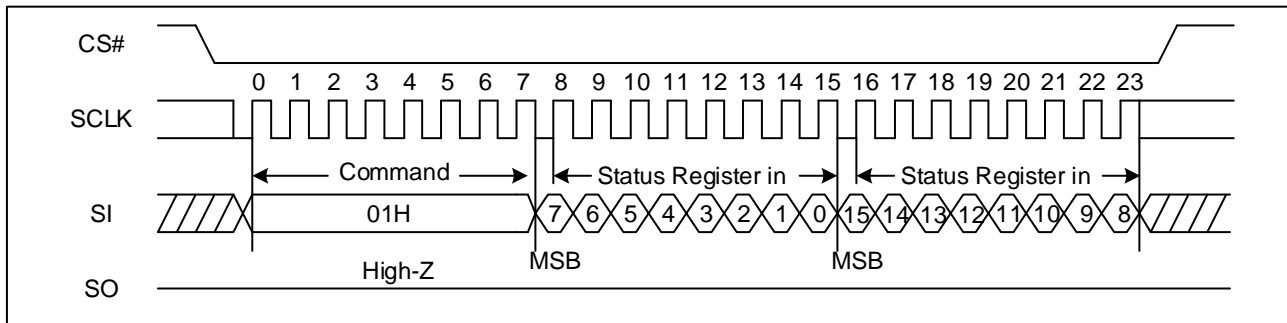
Figure 21. Write Status Register-1&2 Sequence Diagram (SPI)
