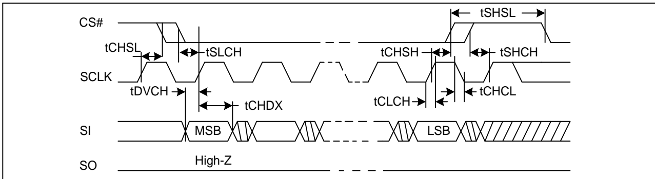
Figure 44. Input Timing
