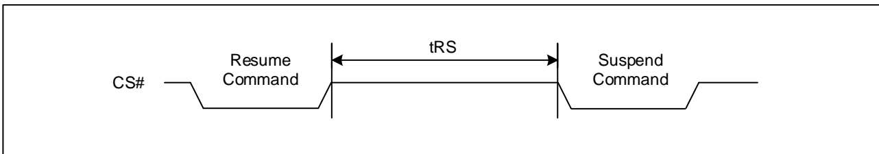
Figure 46. Resume to Suspend Timing Diagram
