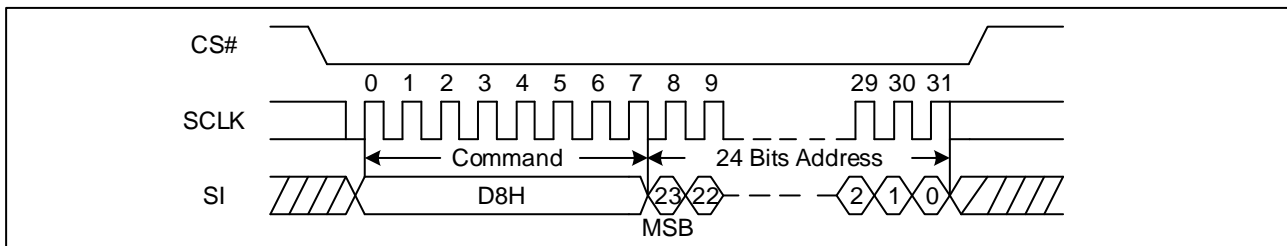
Figure 20. 64KB Block Erase Sequence Diagram (ADS=0)
