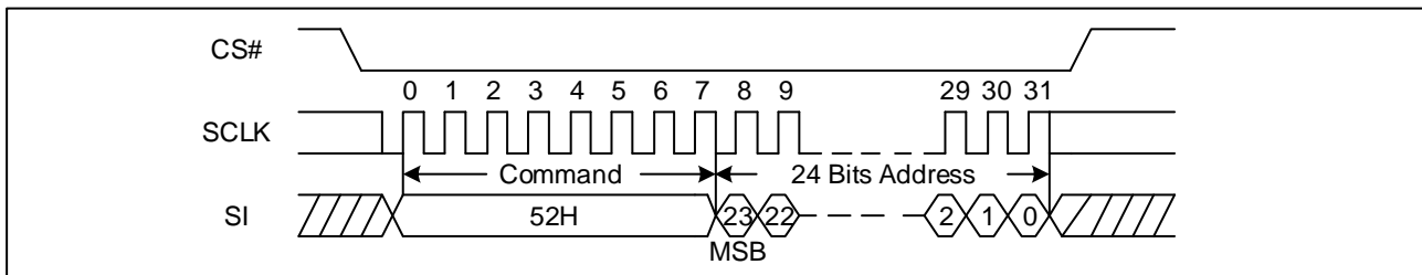
Figure 19. 32KB Block Erase Sequence Diagram (ADS=0)
