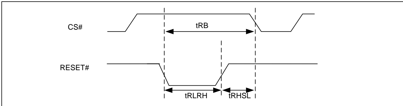
Figure 47 RESET Timing
