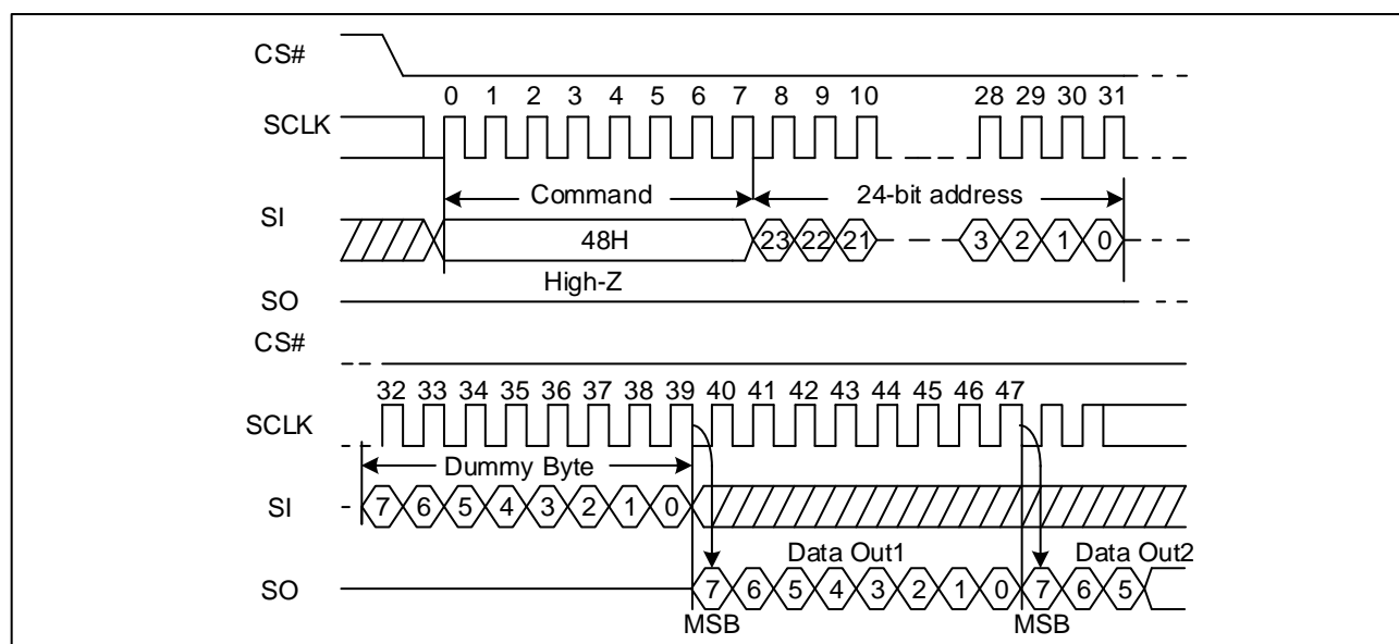
Figure 47. Read Security Registers command Sequence Diagram
