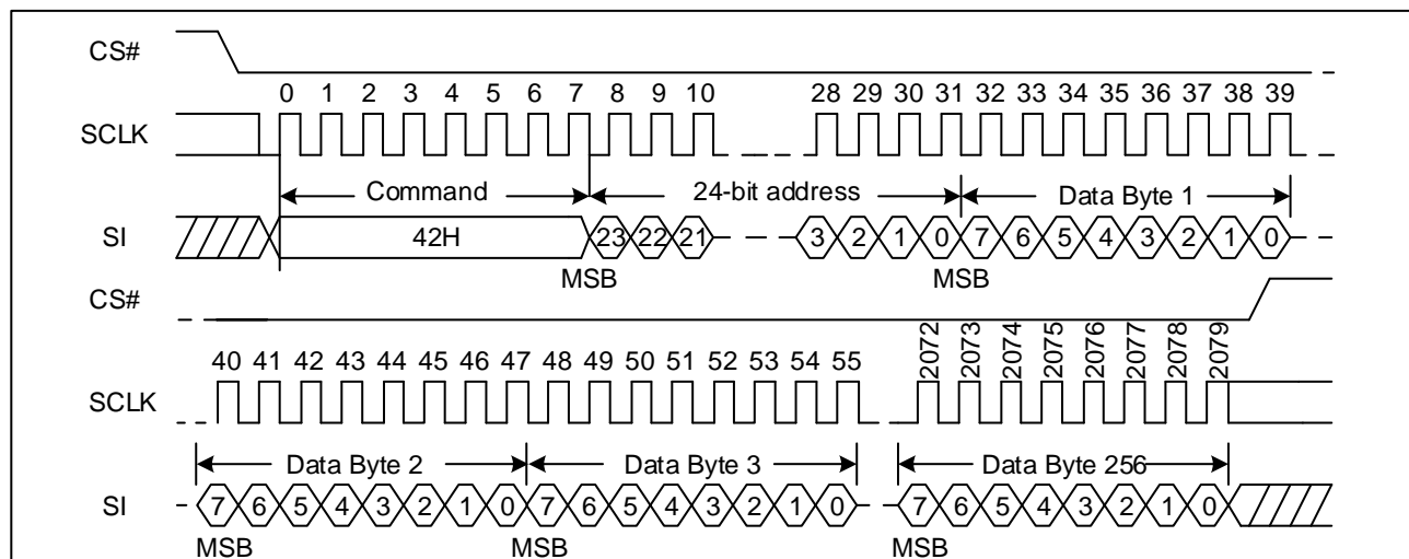
Figure 46. Program Security Registers command Sequence Diagram
