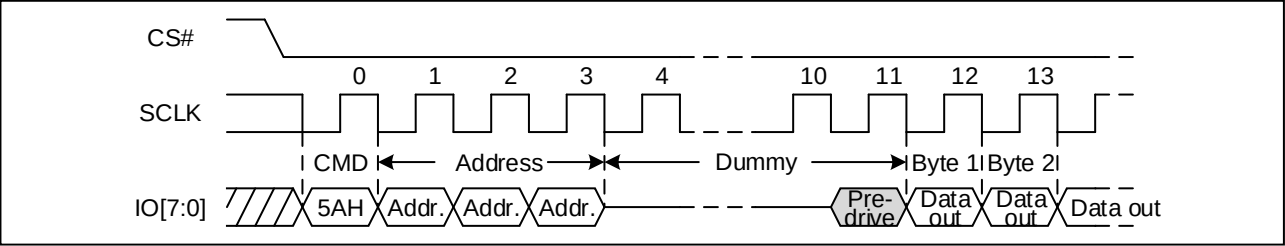
Figure 116. Read Serial Flash Discoverable Parameter command Sequence Diagram (STR OPI)
