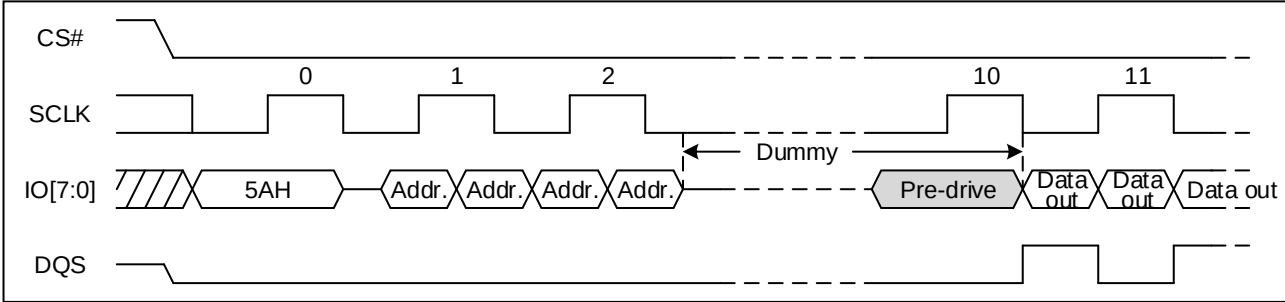
Figure 117. Read Serial Flash Discoverable Parameter command Sequence Diagram (DTR OPI)
