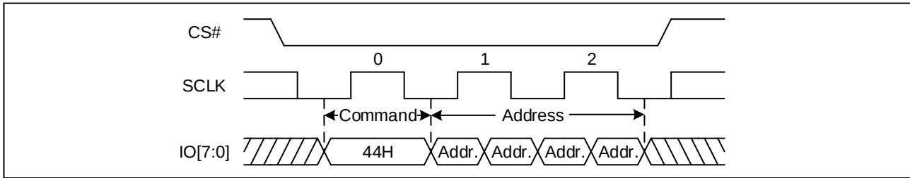
Figure 93. Erase Security Registers command Sequence Diagram (DTR, OPI)
