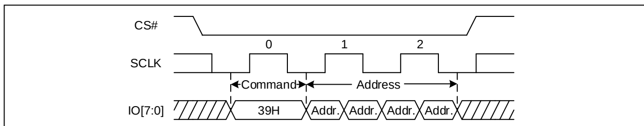
Figure 105. Individual Block/Sector Unlock command Sequence Diagram (DTR OPI)
