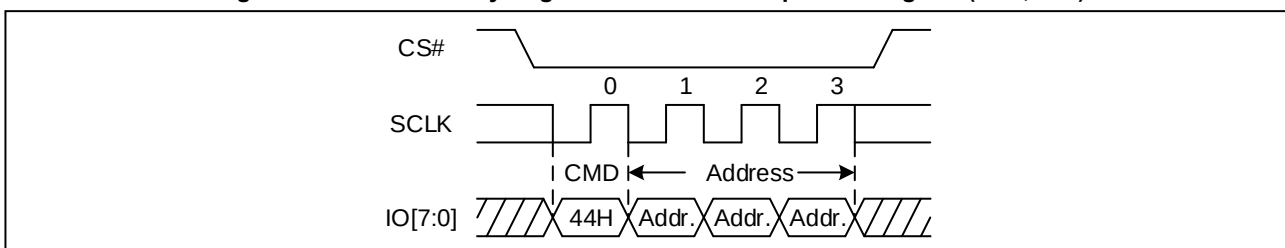
Figure 92. Erase Security Registers command Sequence Diagram (STR, OPI)
