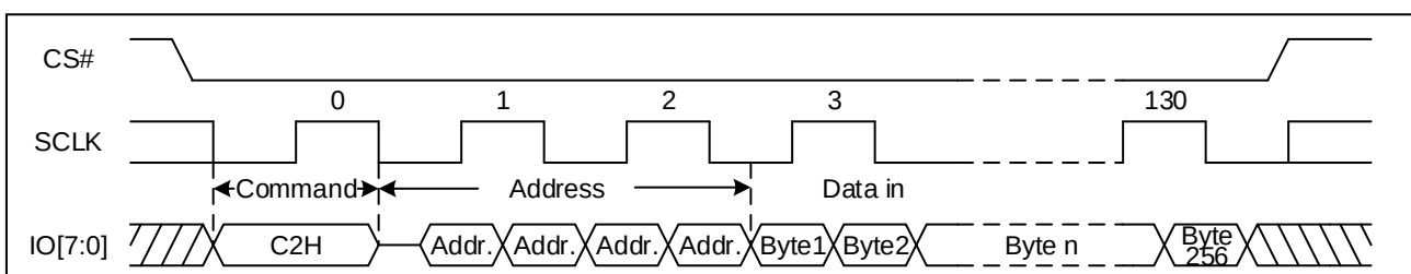
Figure 65. Page Program Sequence Diagram (DTR OPI)
