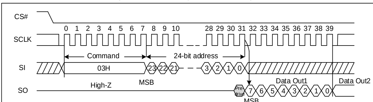
Figure 42. Read Data Bytes Sequence Diagram
