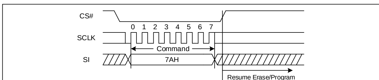
Figure 89. Program/Erase Resume Sequence Diagram (SPI)
