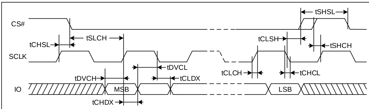
Figure 123. Serial Input Timing (DTR)
