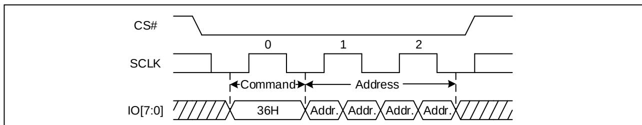
Figure 102. Individual Block/Sector Lock command Sequence Diagram (DTR OPI)
