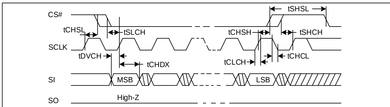
Figure 121. Serial Input Timing
