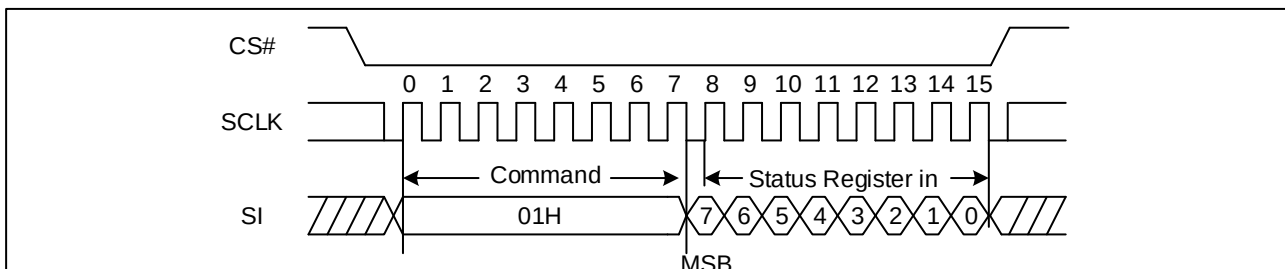
Figure 23. Write Status Register Sequence Diagram (SPI)
