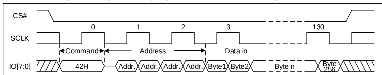
Figure 96. Program Security Registers command Sequence Diagram (DTR OPI)
