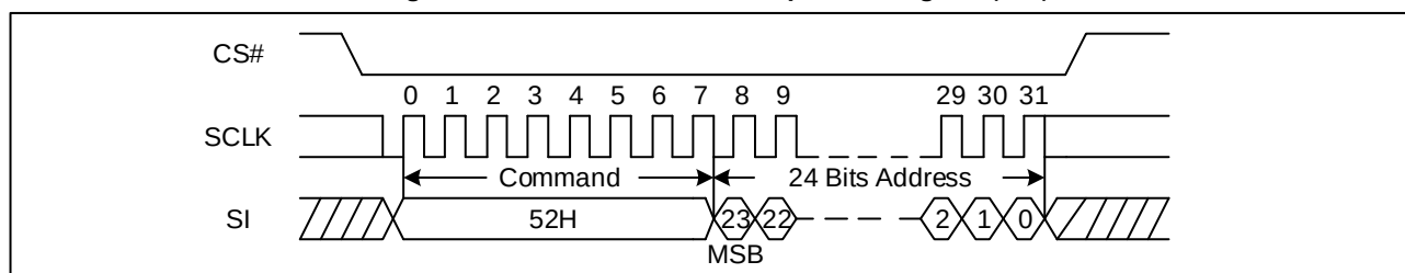
Figure 69. 32KB Block Erase Sequence Diagram (SPI)
