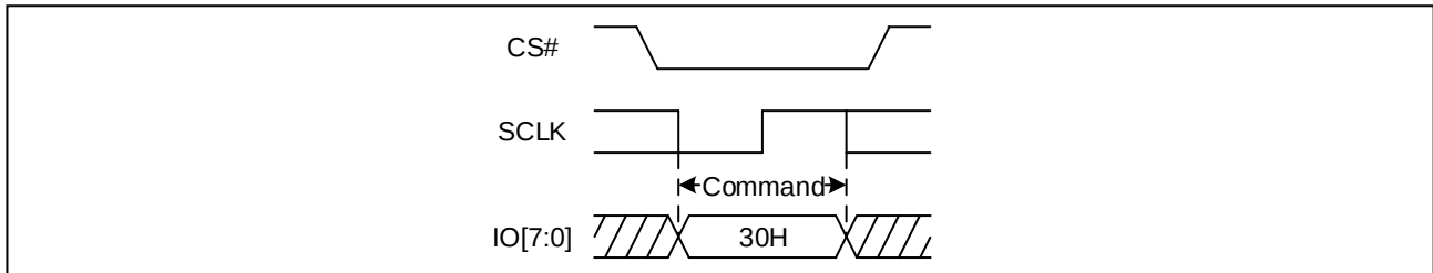
Figure 16. Clear Status Register Flags Diagram (OPI)
