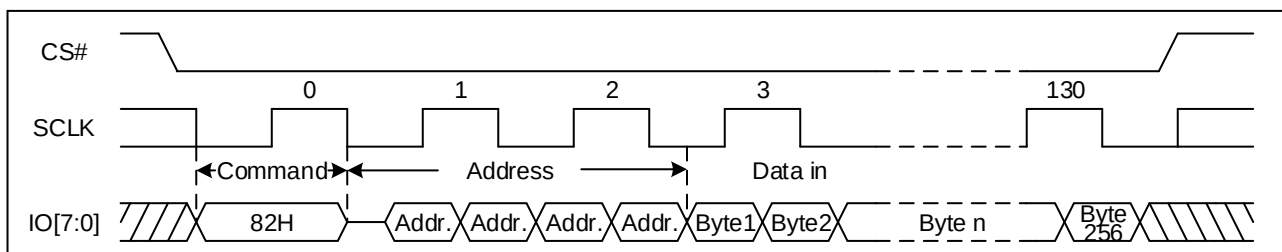
Figure 62. Page Program Sequence Diagram (DTR OPI)
