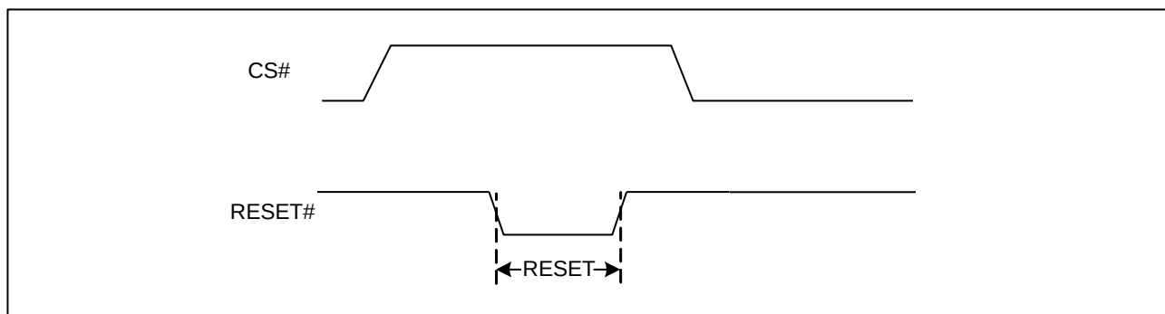
Figure 4 RESET Condition
