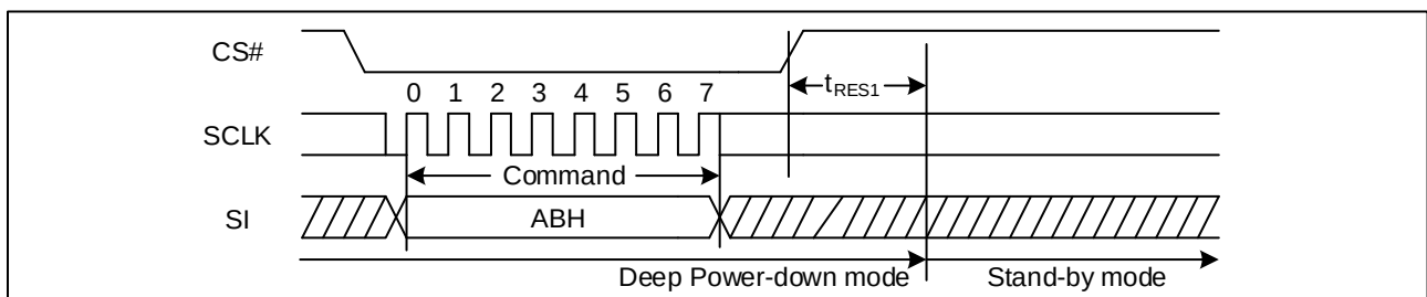
Figure 79. Release Power-Down Sequence Diagram (SPI)
