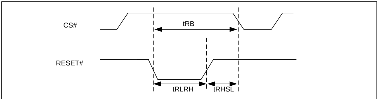
Figure 129. RESET Timing
