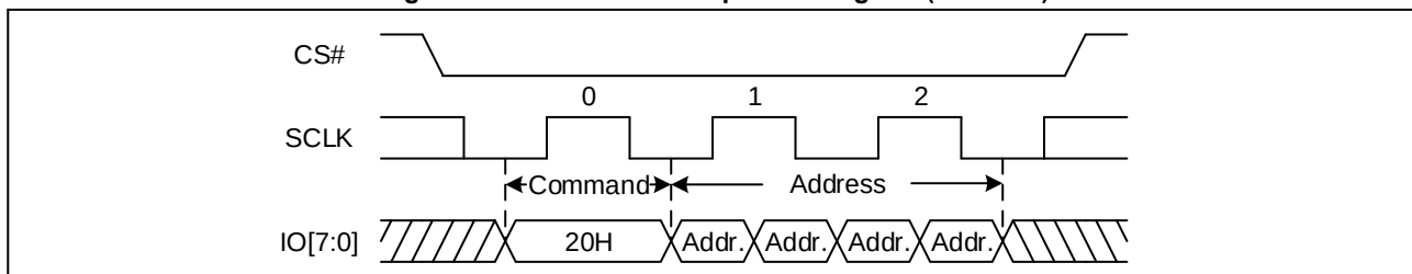
Figure 68. Sector Erase Sequence Diagram (DTR OPI)
