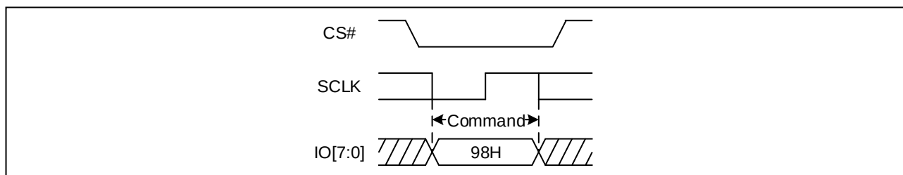
Figure 112. The Global Block/Sector Unlock Sequence Diagram (OPI)
