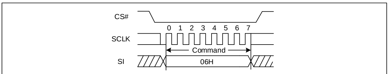
Figure 17. Write Enable Sequence Diagram (SPI)
