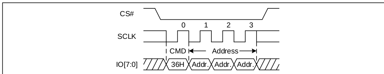
Figure 101. Individual Block/Sector Lock command Sequence Diagram (STR OPI)
