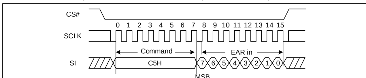
Figure 25. Write Extended Address Register Sequence Diagram (SPI)
