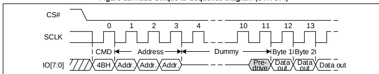
Figure 82. Read Unique ID Sequence Diagram (STR OPI)
