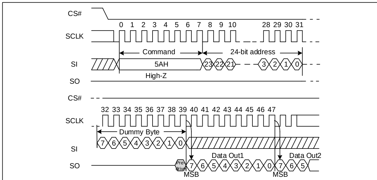
Figure 115. Read Serial Flash Discoverable Parameter command Sequence Diagram (SPI)
