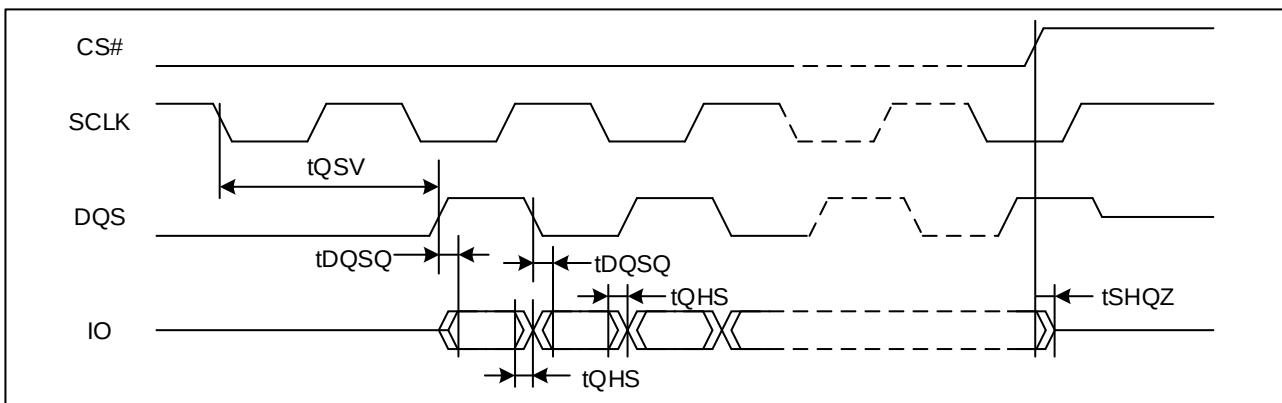
Figure 126. DQS Output Timing (DTR)
