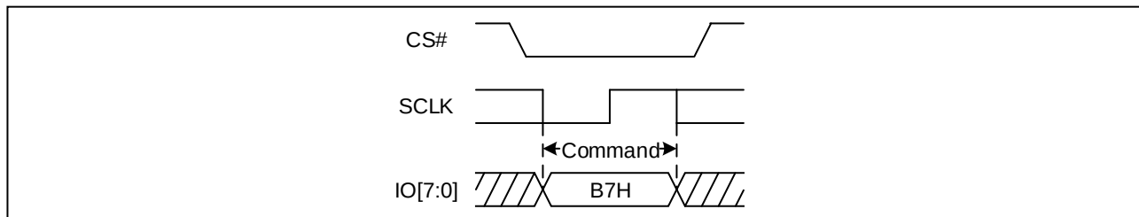
Figure 12. Enable 4-Byte Mode Sequence Diagram (OPI)
