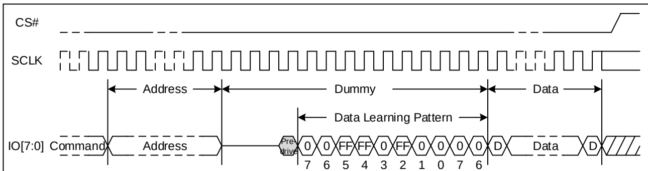
Figure 7. Data Learning Pattern Sequence Diagram (STR, Dummy Clock \geq 12 )
