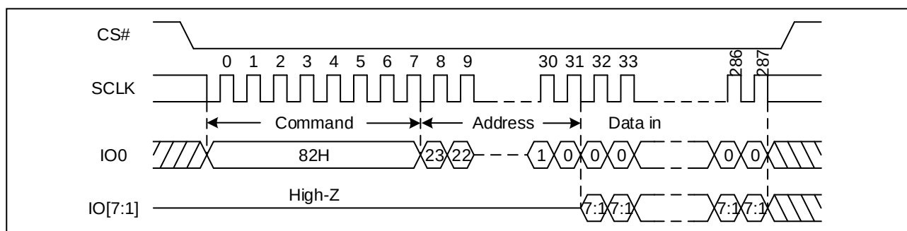
Figure 60. Octal Page Program Sequence Diagram (SPI)
