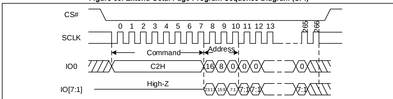
Figure 63. Extend Octal Page Program Sequence Diagram (SPI)
