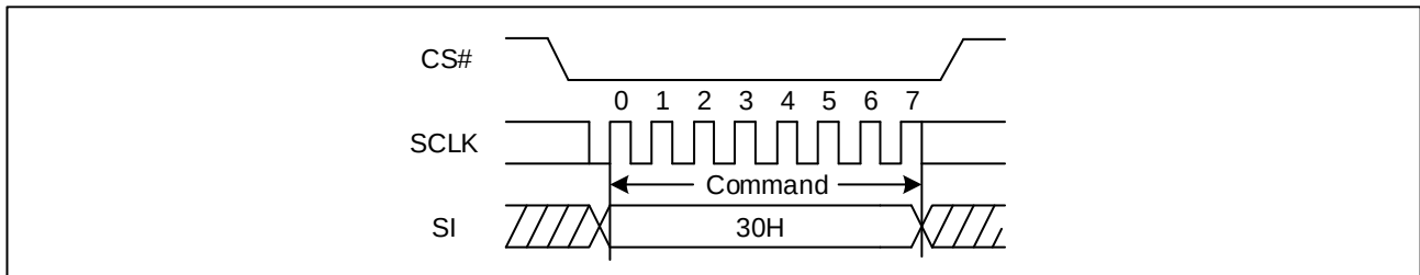
Figure 15. Clear Status Register Flags Diagram (SPI)
