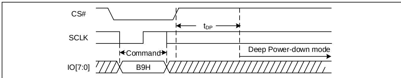
Figure 78. Deep Power-Down Sequence Diagram (OPI)
