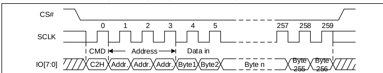
Figure 64. Page Program Sequence Diagram (STR OPI)
