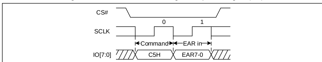
Figure 26. Write Extended Address Register Sequence Diagram (OPI)
