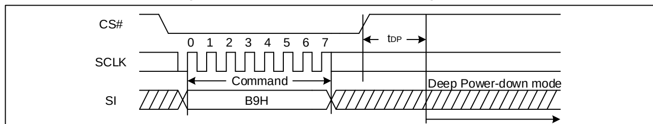
Figure 77. Deep Power-Down Sequence Diagram (SPI)
