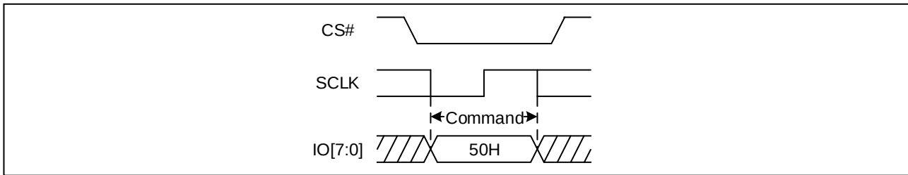
Figure 22. Write Enable for Volatile Status Register Sequence Diagram (OPI)
