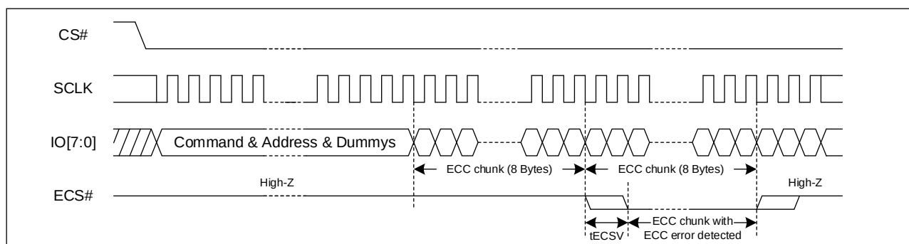
Figure 5. ECS# Timing
