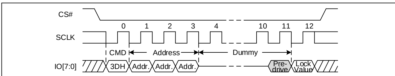
Figure 107. Read Individual Block/Sector lock command Sequence Diagram (STR OPI)
