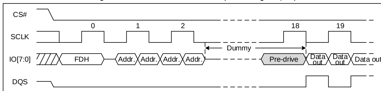
Figure 55. Octal I/O DTR Fast Read Sequence Diagram (OPI)
