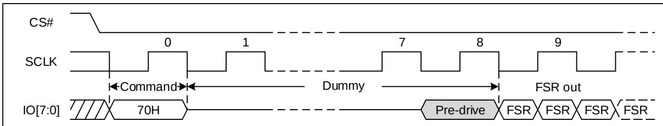
Figure 35. Read Flag Status Register Sequence (DTR OPI)
