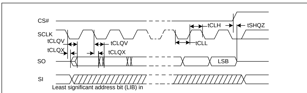
Figure 122. Output Timing
