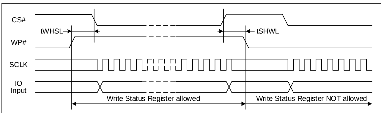
Figure 128. WP# Timing
