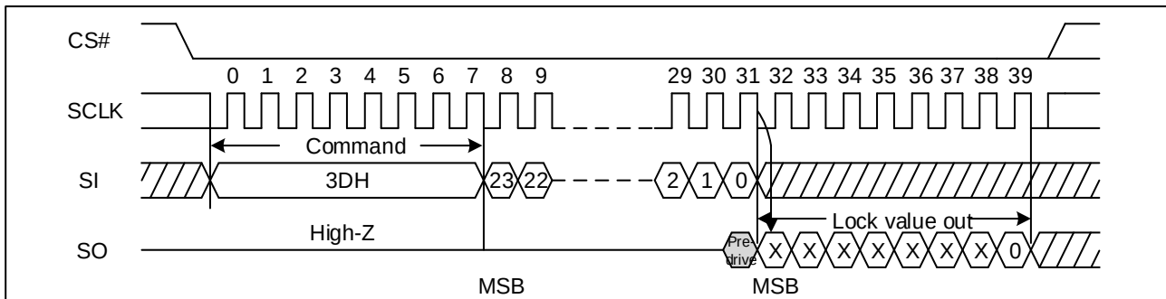
Figure 106. Read Individual Block/Sector lock command Sequence Diagram (SPI)
