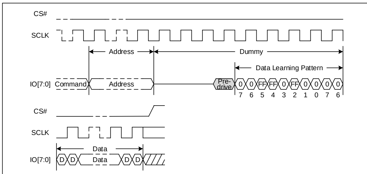
Figure 9. Data Learning Pattern Sequence Diagram (DTR, Dummy Clock ≥ 8)
