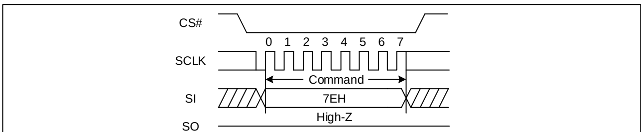
Figure 109. The Global Block/Sector Lock Sequence Diagram (SPI)
