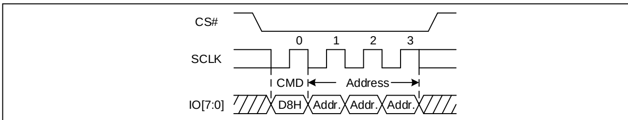
Figure 73. 64KB Block Sequence Diagram (STR OPI)
