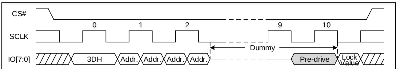
Figure 108. Read Individual Block/Sector lock command Sequence Diagram (DTR OPI)
