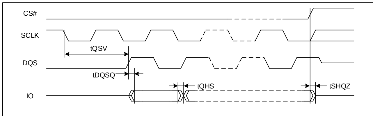
Figure 125. DQS Output Timing (STR)
