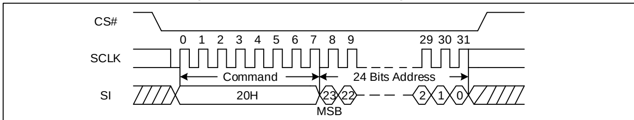
Figure 66. Sector Erase Sequence Diagram (SPI)
