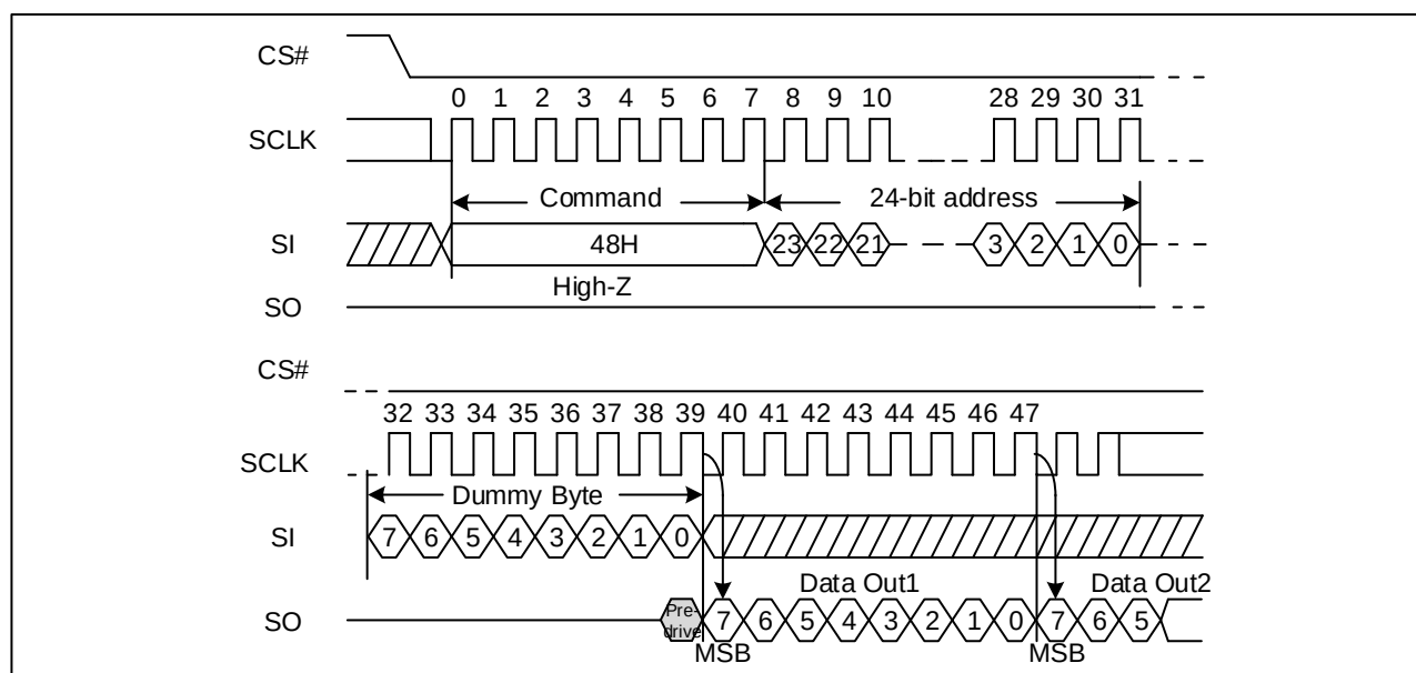
Figure 97. Read Security Registers command Sequence Diagram (SPI)
