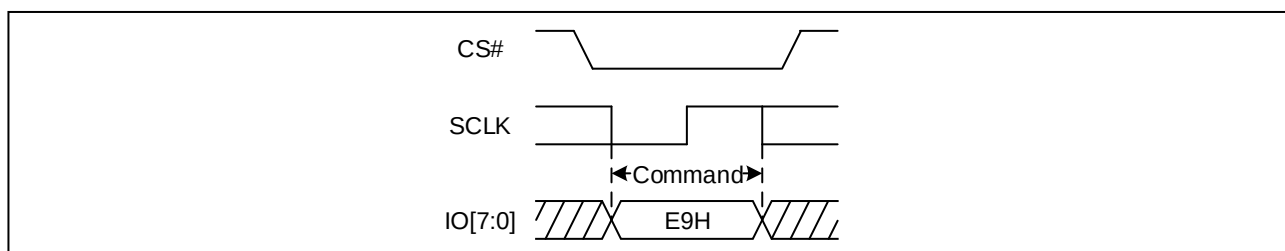
Figure 14. Disable 4-Byte Mode Sequence Diagram (OPI)
