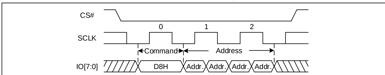
Figure 74. 64KB Block Sequence Diagram (DTR OPI)
