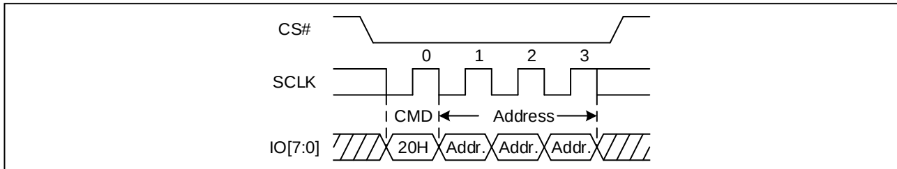
Figure 67. Sector Erase Sequence Diagram (STR OPI)
