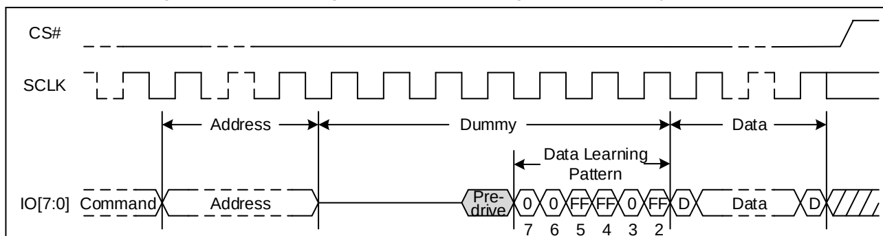
Figure 10. Data Learning Pattern Sequence Diagram (DTR, Dummy Clock < 8)
