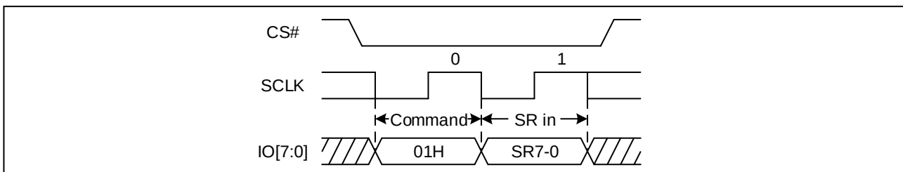
Figure 24. Write Status Register Sequence Diagram (OPI)
