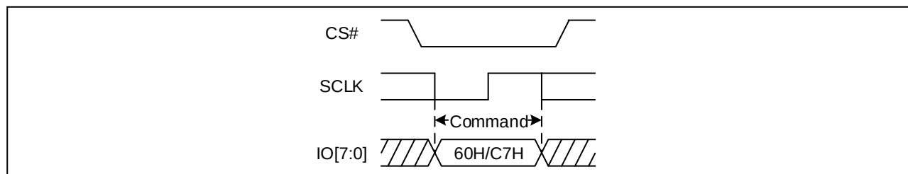
Figure 76. Chip Erase Sequence Diagram (OPI)
