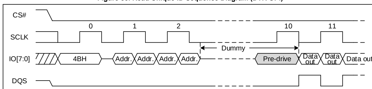
Figure 83. Read Unique ID Sequence Diagram (DTR OPI)
