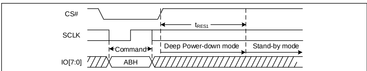
Figure 80. Release Power-Down Sequence Diagram (OPI)
