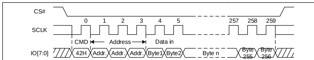
Figure 95. Program Security Registers command Sequence Diagram (STR OPI)
