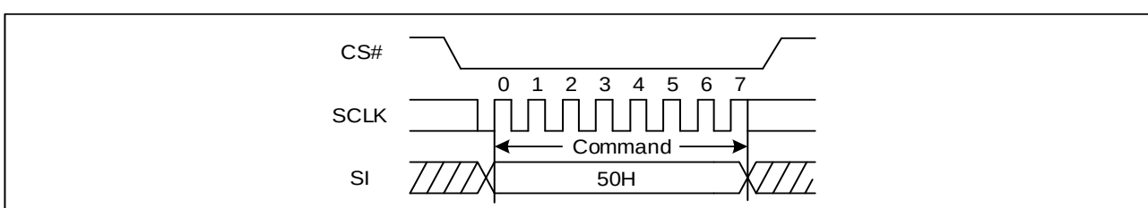
Figure 21. Write Enable for Volatile Status Register Sequence Diagram (SPI)
