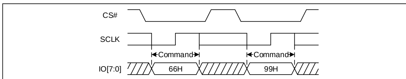
Figure 114. Enable Reset and Reset command Sequence Diagram (OPI)
