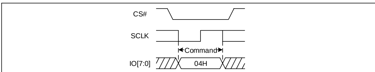
Figure 20. Write Disable Sequence Diagram (OPI)
