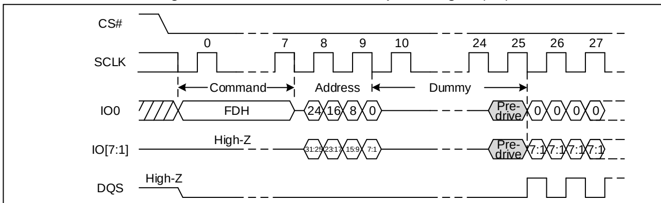
Figure 54. Octal I/O DTR Fast Read Sequence Diagram (SPI)
