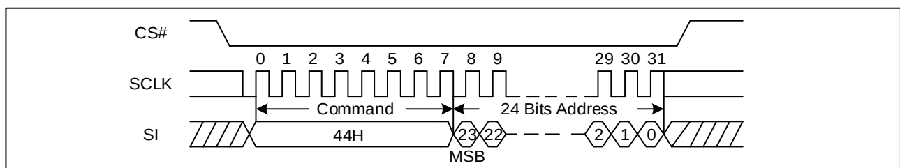
Figure 91. Erase Security Registers command Sequence Diagram (SPI)
