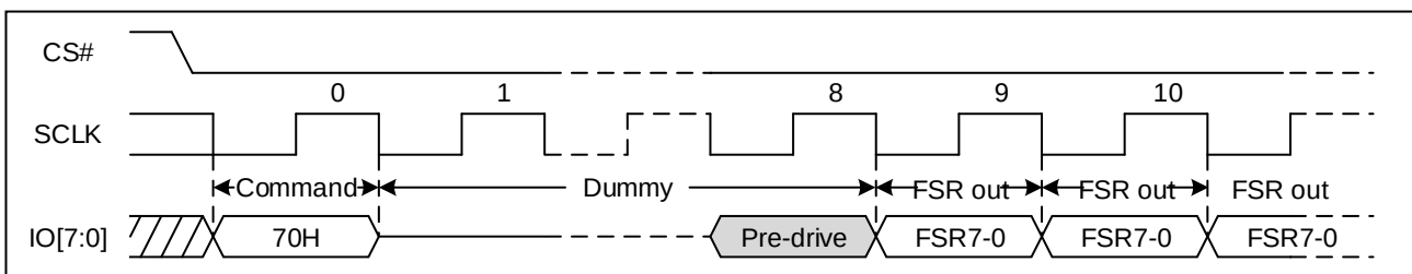
Figure 34. Read Flag Status Register Sequence (STR OPI)
