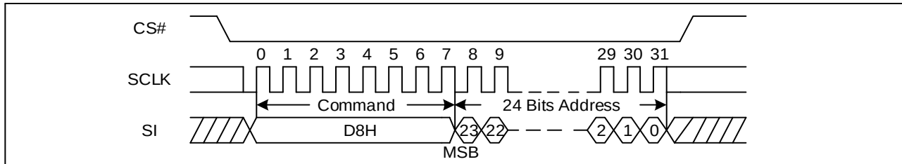
Figure 72. 64KB Block Erase Sequence Diagram (SPI)
