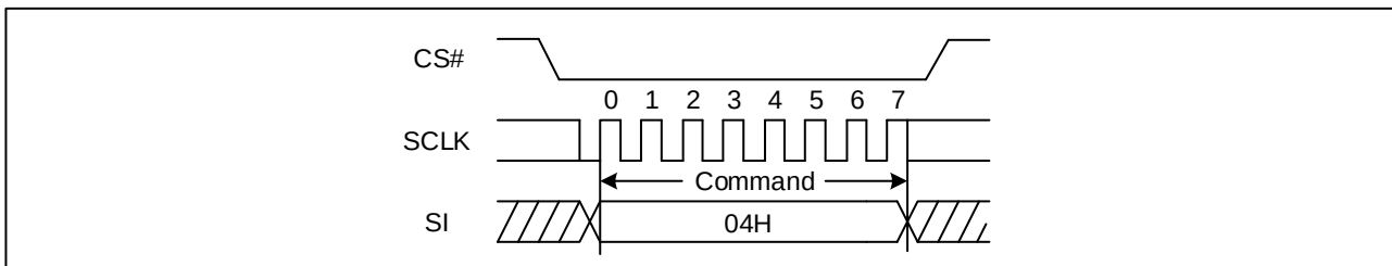
Figure 19. Write Disable Sequence Diagram (SPI)
