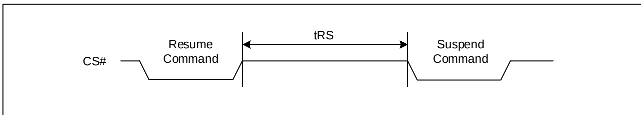
Figure 127. Resume to Suspend Timing Diagram
