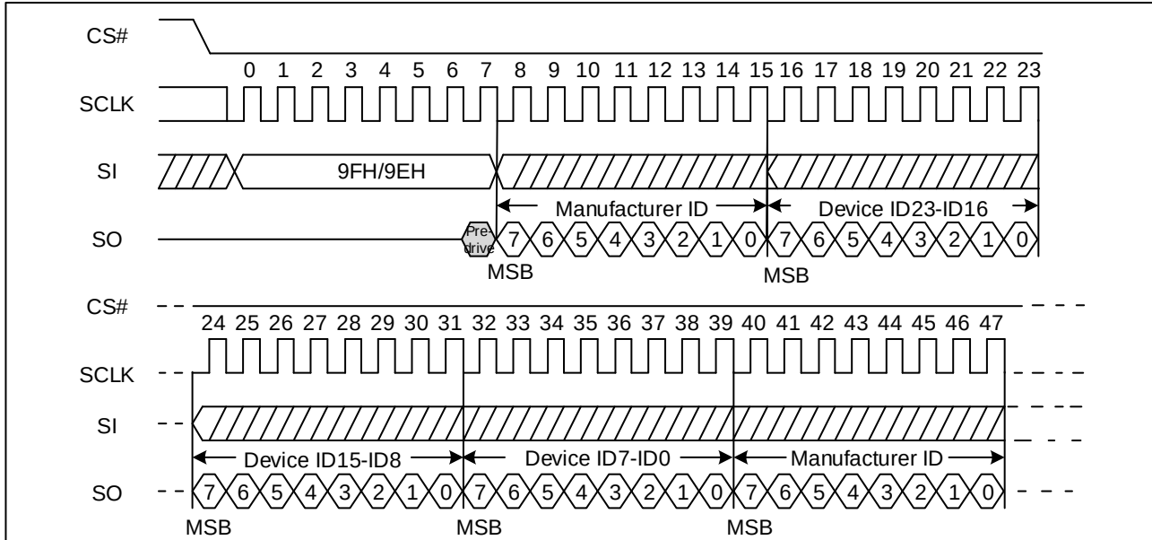
Figure 84. Read Identification ID Sequence Diagram (SPI)
