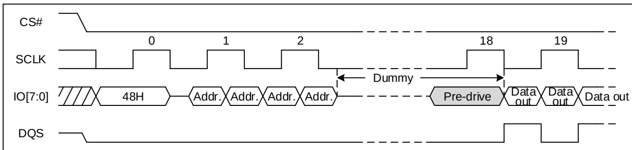
Figure 99. Read Security Registers command Sequence Diagram (DTR OPI)
