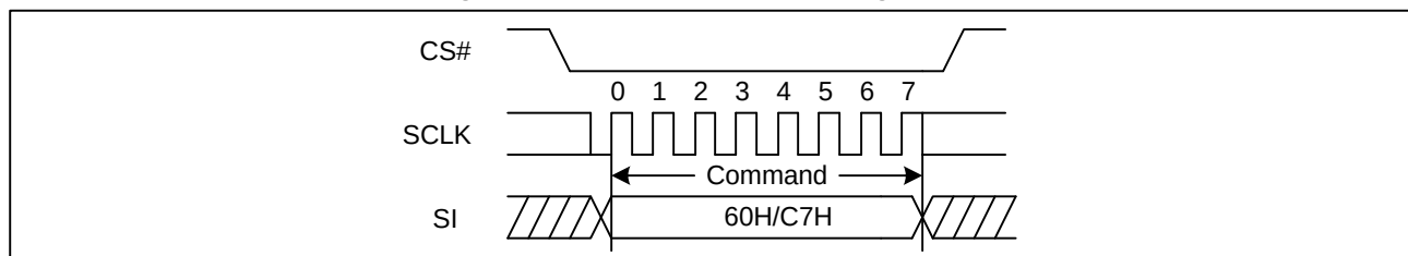
Figure 75 Chip Erase Sequence Diagram (SPI)
