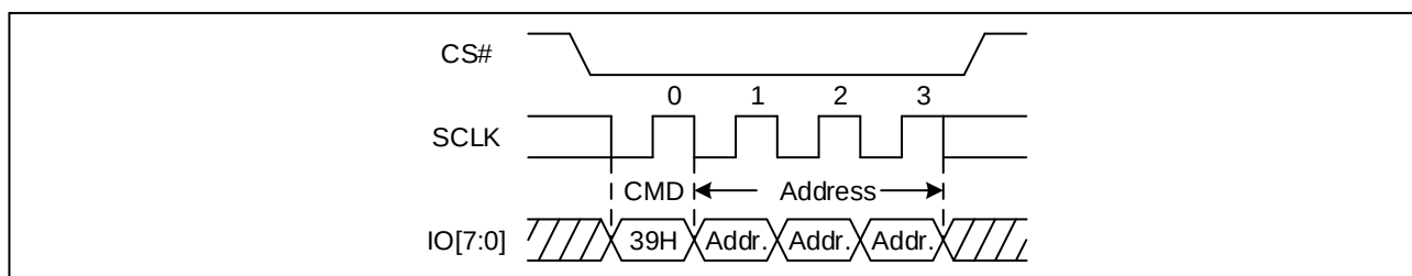
Figure 104. Individual Block/Sector Unlock command Sequence Diagram (STR OPI)
