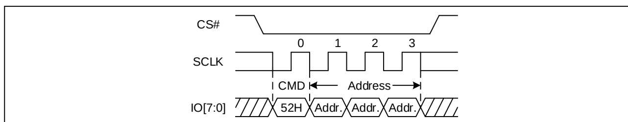
Figure 70. 32KB Block Erase Sequence Diagram (STR OPI)
