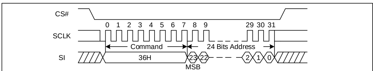
Figure 100. Individual Block/Sector Lock command Sequence Diagram (SPI)
