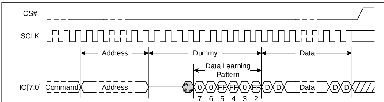
Figure 8. Data Learning Pattern Sequence Diagram (STR, Dummy Clock < 12 )
