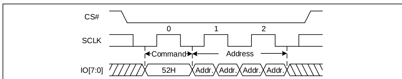
Figure 71. 32KB Block Erase Sequence Diagram (DTR OPI)
