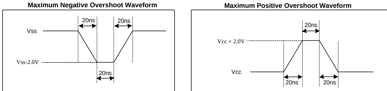
Figure 119. Input Test Waveform and Measurement Level
