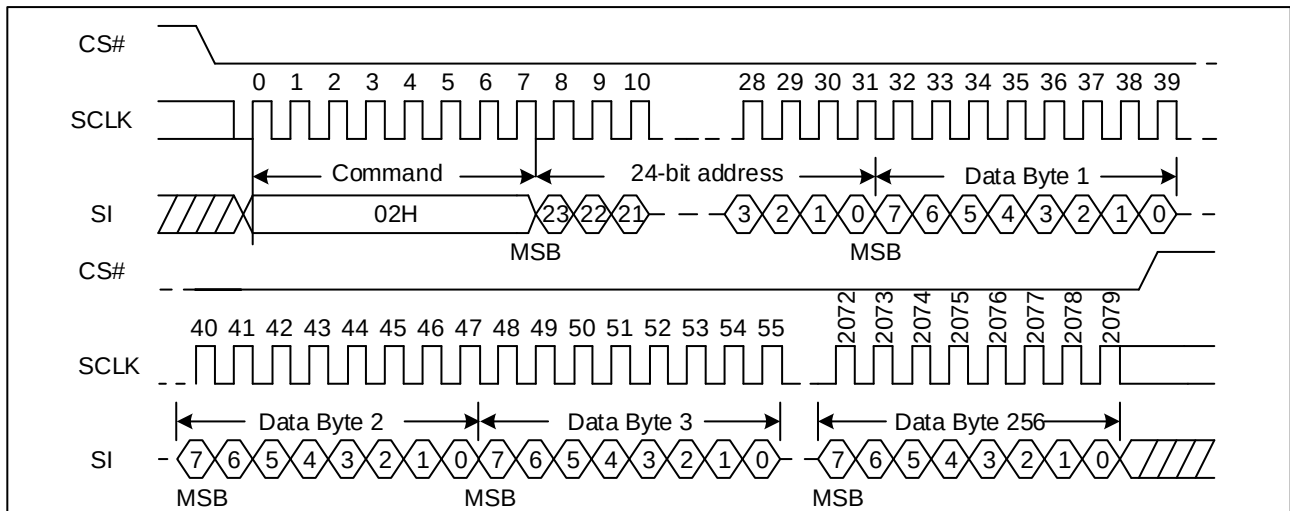
Figure 57. Page Program Sequence Diagram (SPI)
