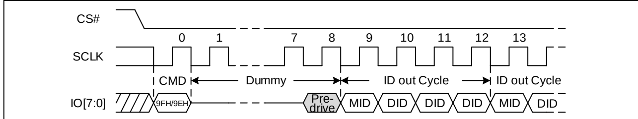
Figure 85. Read Identification ID Sequence Diagram (STR, OPI)
