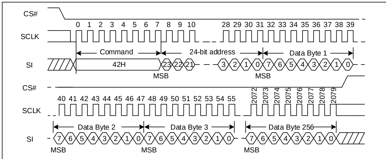
Figure 94. Program Security Registers command Sequence Diagram (SPI)
