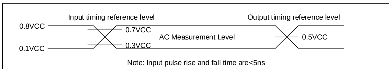
Figure 120. Absolute Maximum Ratings Diagram
