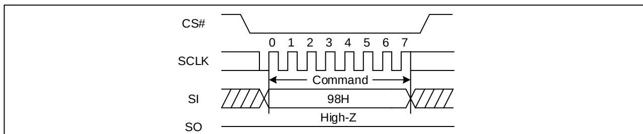
Figure 111. The Global Block/Sector Unlock Sequence Diagram (SPI)
