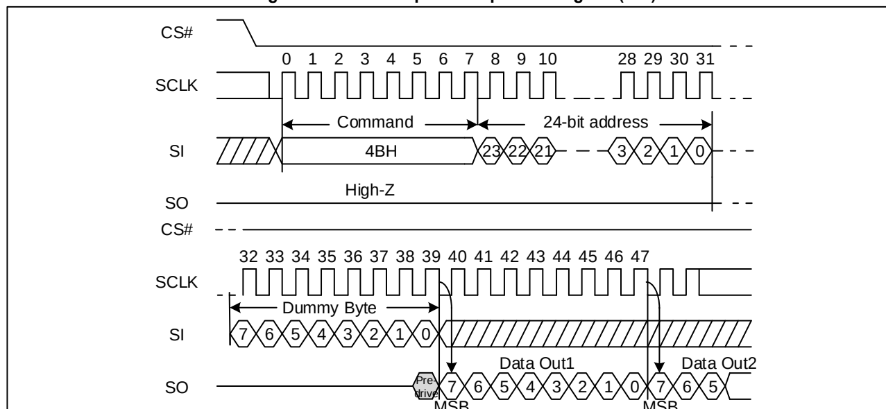
Figure 81. Read Unique ID Sequence Diagram (SPI)
