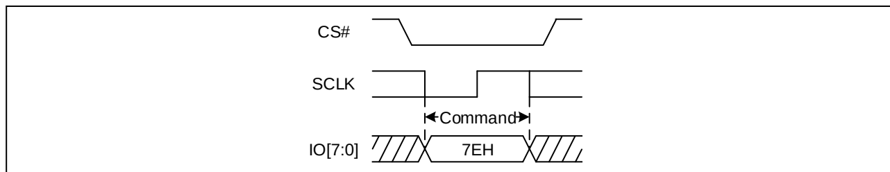
Figure 110. The Global Block/Sector Lock Sequence Diagram (OPI)
