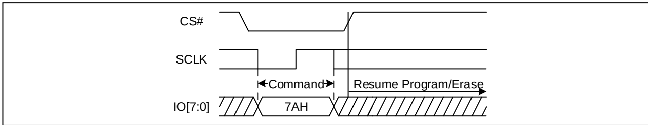
Figure 90. Program/Erase Resume Sequence Diagram (OPI)
