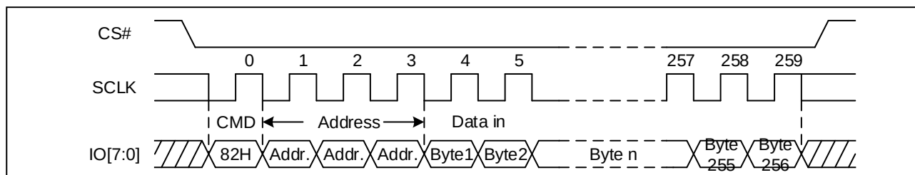
Figure 61. Page Program Sequence Diagram (STR OPI)
