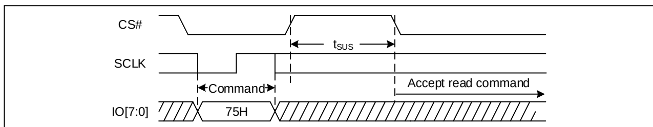
Figure 88. Program/Erase Suspend Sequence Diagram (OPI)
