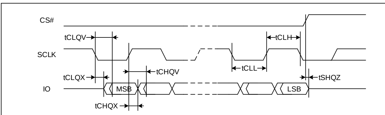
Figure 124. Serial Output Timing (DTR)
