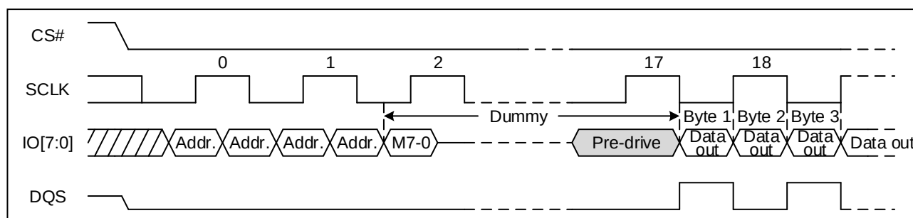
Figure 56. Octal I/O DTR Fast Read Sequence Diagram (M5-4 = (1, 0))
