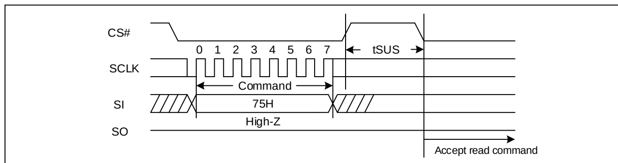
Figure 87. Program/Erase Suspend Sequence Diagram (SPI)
