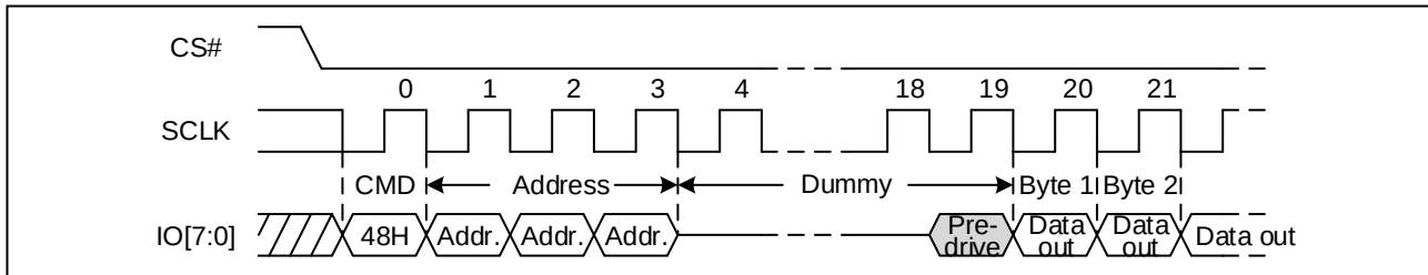
Figure 98. Read Security Registers command Sequence Diagram (STR OPI)
