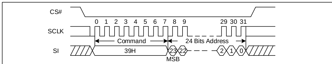
Figure 103. Individual Block/Sector Unlock command Sequence Diagram (SPI)
