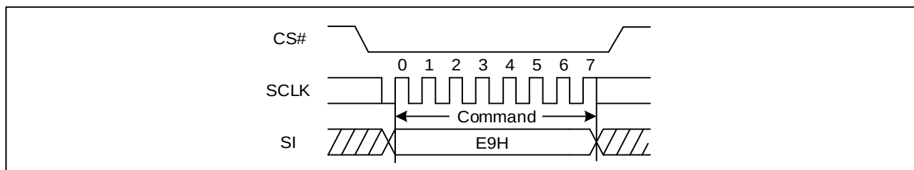
Figure 13. Disable 4-Byte Mode Sequence Diagram (SPI)
