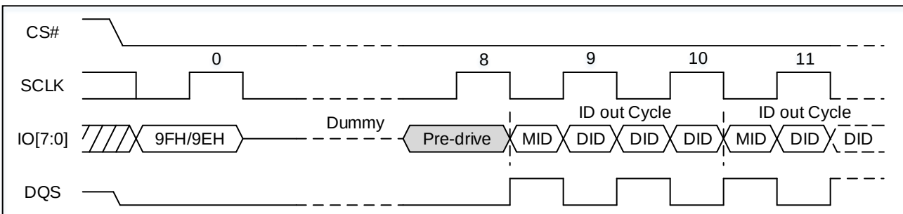
Figure 86. Read Identification ID Sequence Diagram (DTR, OPI)
