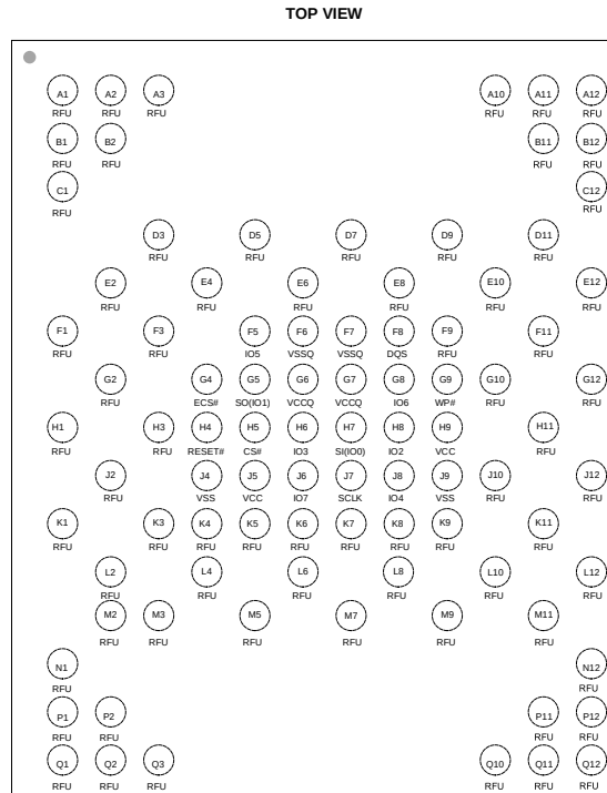
Figure 3 Connection Diagram for WLCSP package
