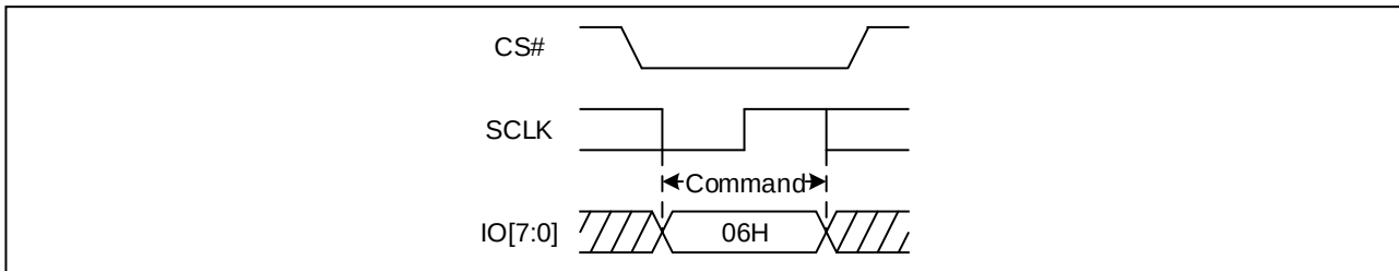
Figure 18. Write Enable Sequence Diagram (OPI)
