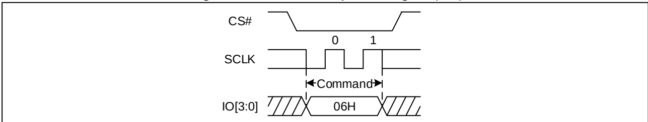
Figure 4. Write Enable Sequence Diagram (QPI)
