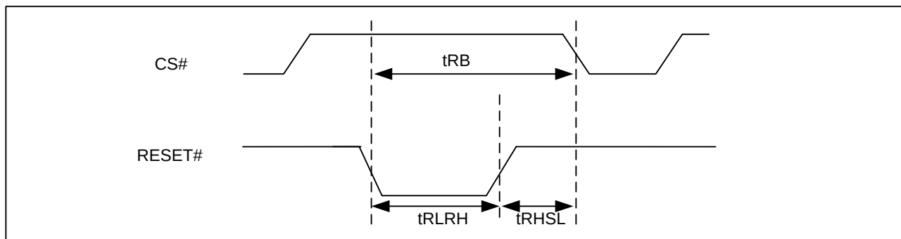
Figure 68 RESET Timing
