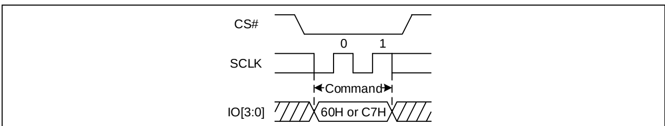
Figure 34. Chip Erase Sequence Diagram (QPI)
