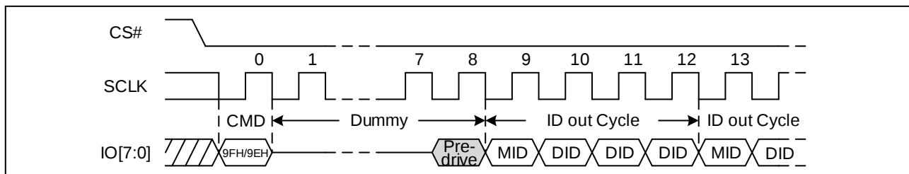
Figure 85. Read Identification ID Sequence Diagram (STR, OPI)
