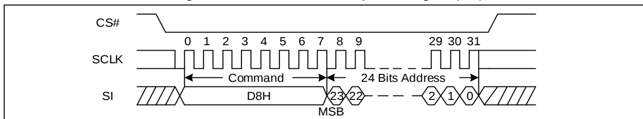
Figure 72. 64KB Block Erase Sequence Diagram (SPI)
