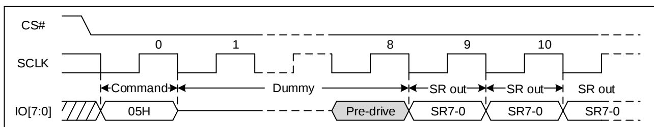
Figure 31. Read Status Register Sequence (STR OPI)
