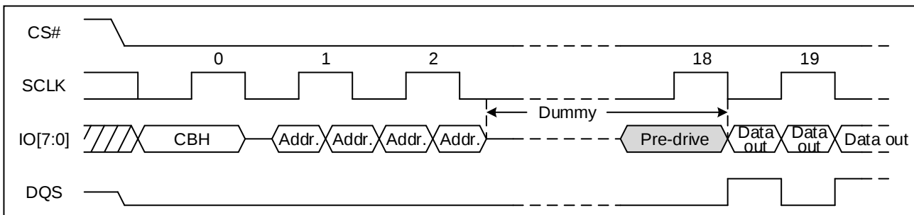
Figure 51. Octal I/O Fast Read Sequence Diagram (DTR OPI, M5-4 \neq (1, 0))
