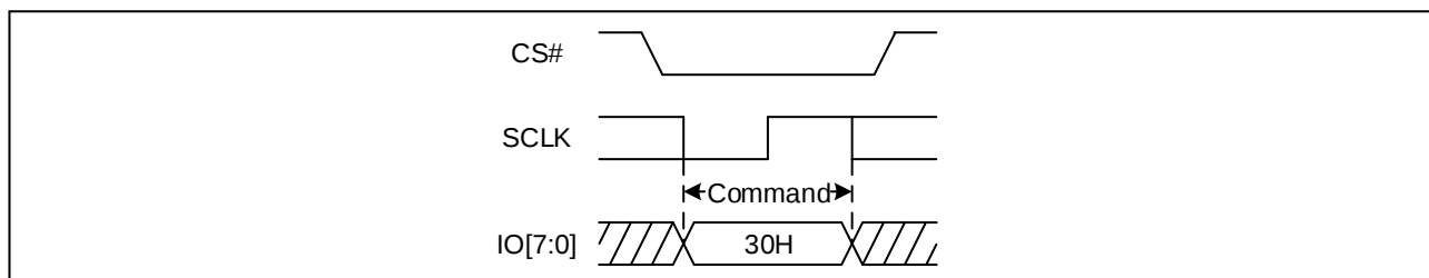
Figure 16. Clear Status Register Flags Diagram (QPI)
