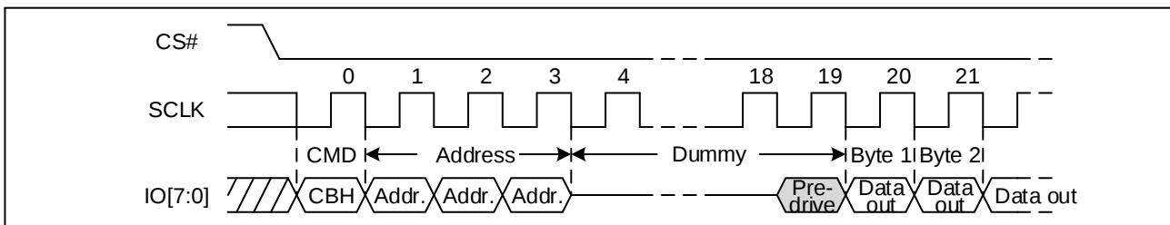
Figure 50. Octal I/O Fast Read Sequence Diagram (STR OPI, M5-4 \neq (1, 0))
