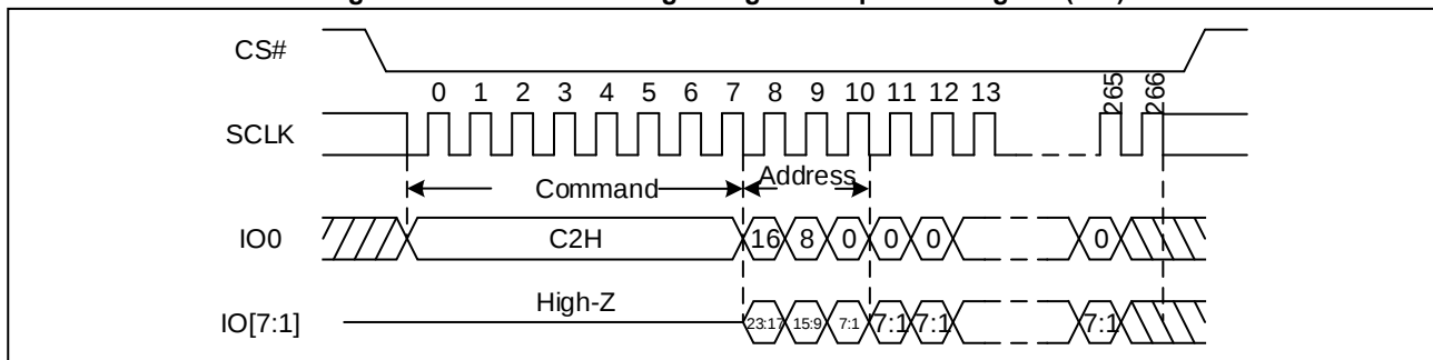
Figure 63. Extend Octal Page Program Sequence Diagram (SPI)
