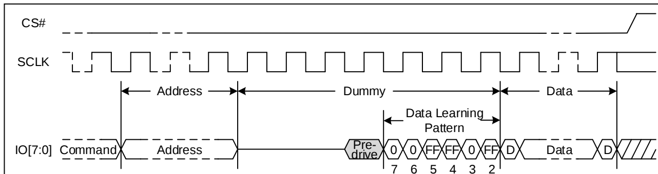
Figure 10. Data Learning Pattern Sequence Diagram (DTR, Dummy Clock < 8)
