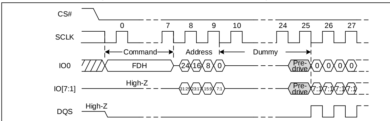
Figure 54. Octal I/O DTR Fast Read Sequence Diagram (SPI)
