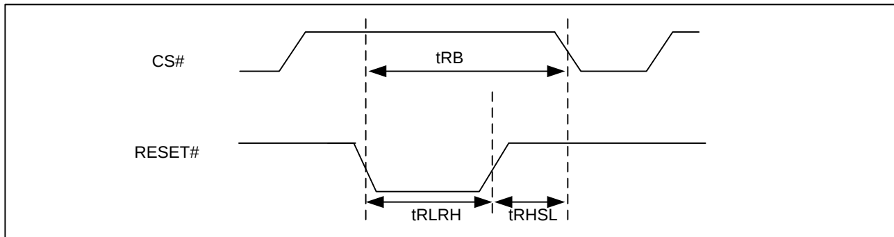
Figure 129. RESET Timing
