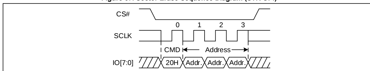
Figure 67. Sector Erase Sequence Diagram (STR OPI)
