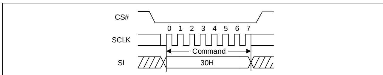
Figure 15. Clear Status Register Flags Diagram (SPI)
