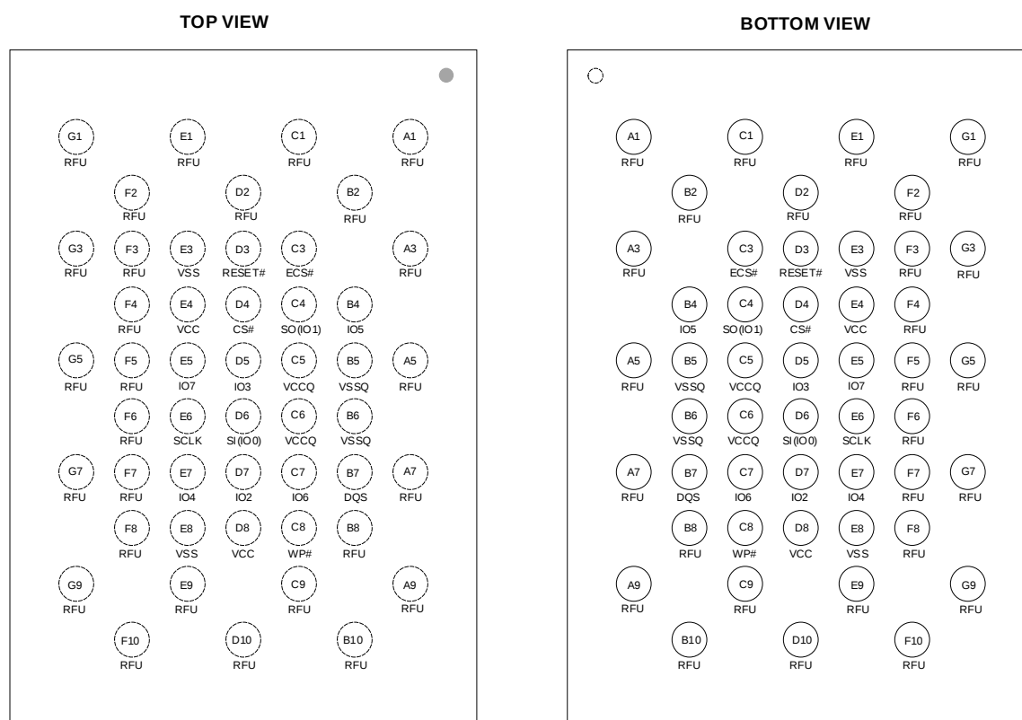
Figure 3 Connection Diagram for WLCSP (4x6 ball array) package
