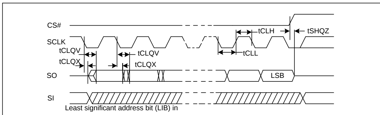
Figure 122. Output Timing
