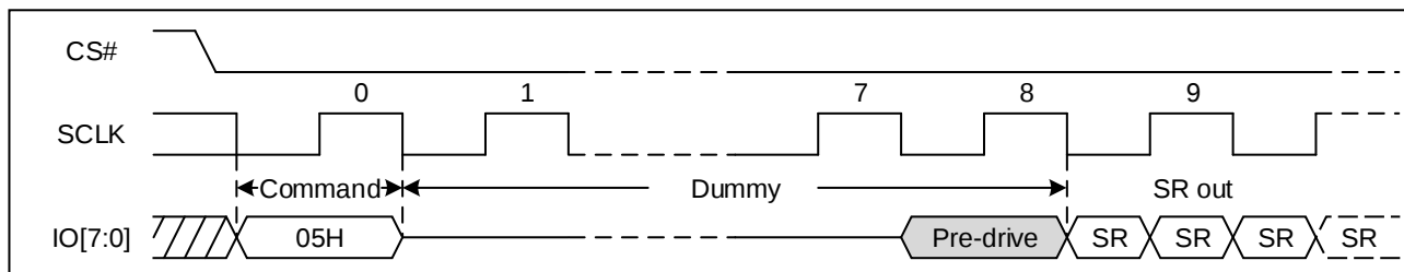
Figure 32. Read Status Register Sequence (DTR OPI)
