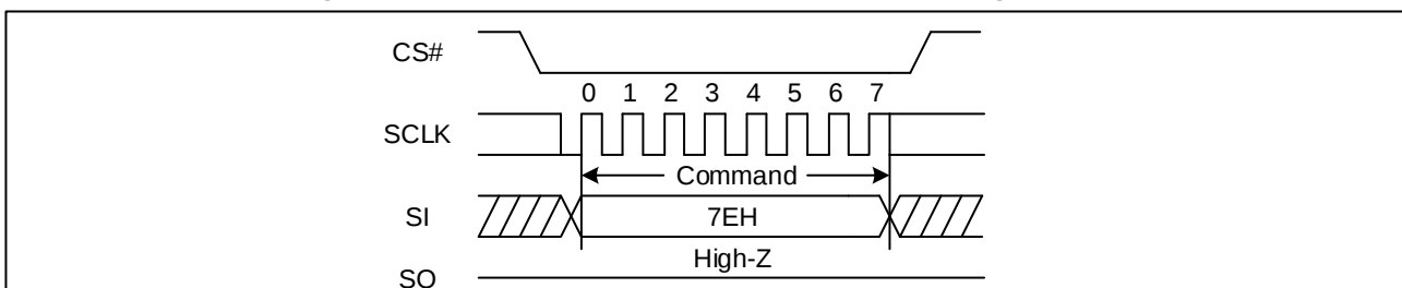
Figure 109. The Global Block/Sector Lock Sequence Diagram (SPI)
