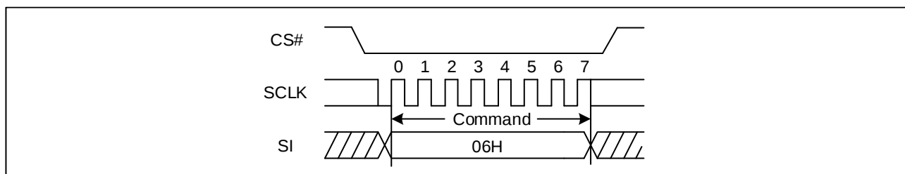
Figure 17. Write Enable Sequence Diagram (SPI)
