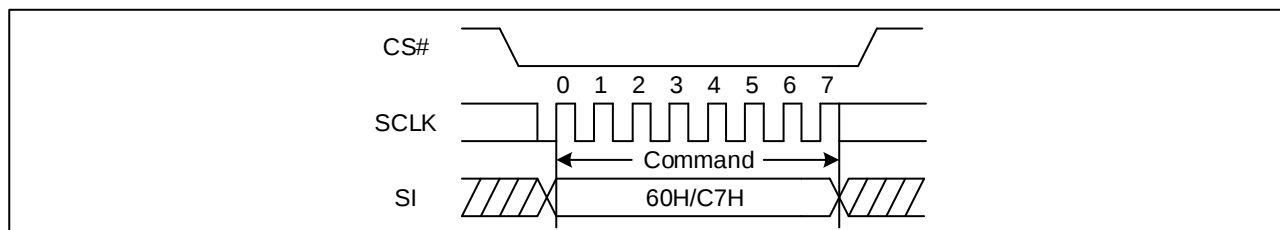
Figure 75. Chip Erase Sequence Diagram (SPI)
