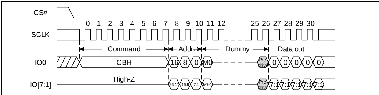
Figure 49. Octal I/O Fast Read Sequence Diagram (SPI, M5-4 \neq (1, 0))
