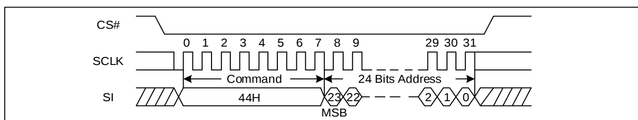
Figure 91. Erase Security Registers command Sequence Diagram (SPI)
