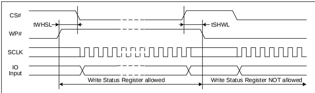
Figure 128. WP# Timing
