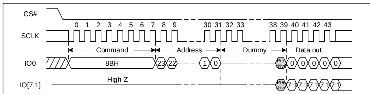
Figure 46. Octal Output Fast Read Sequence Diagram (SPI)
